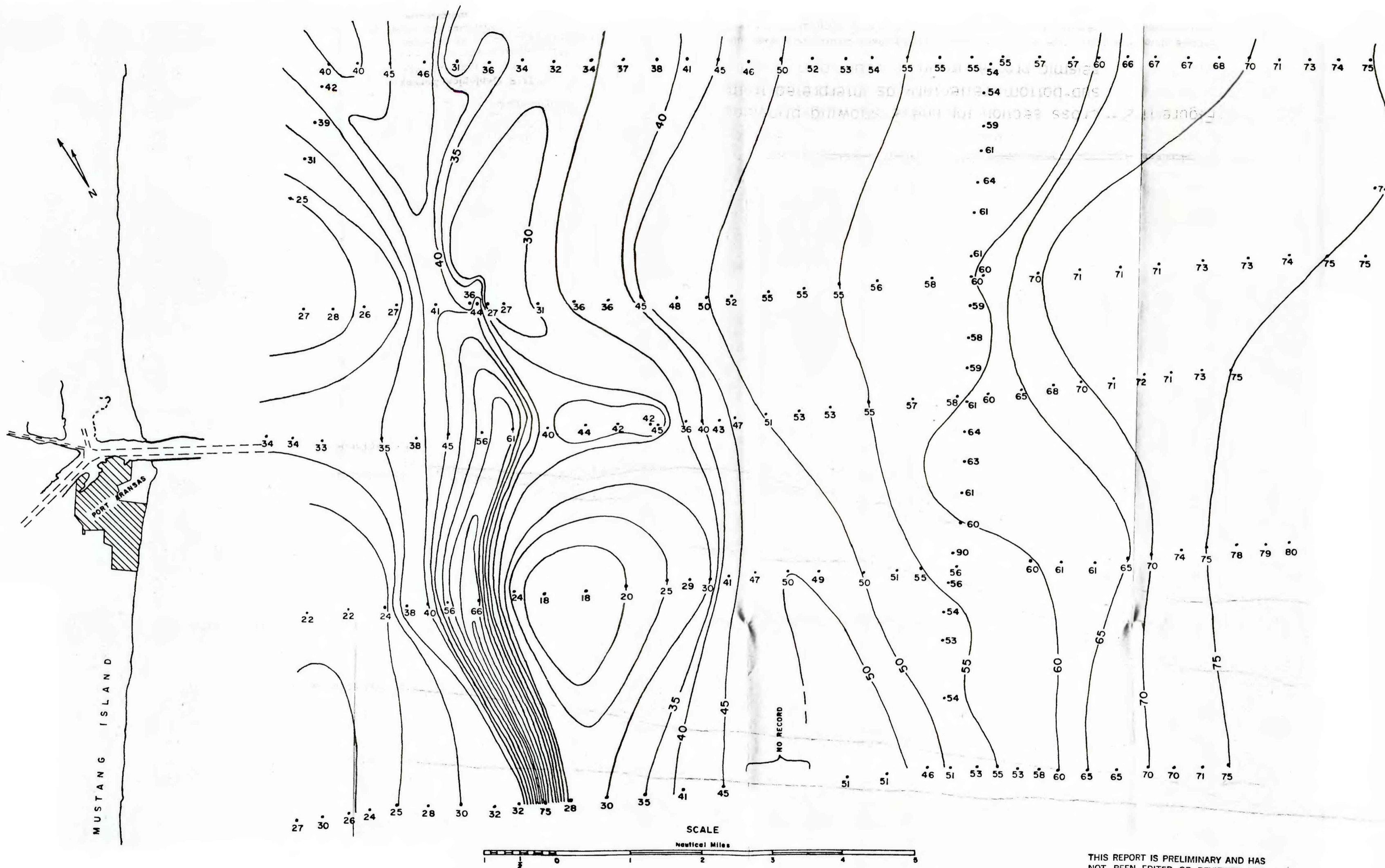
Figure 11b--Thickness of sediments from sea floor to reflector A.
