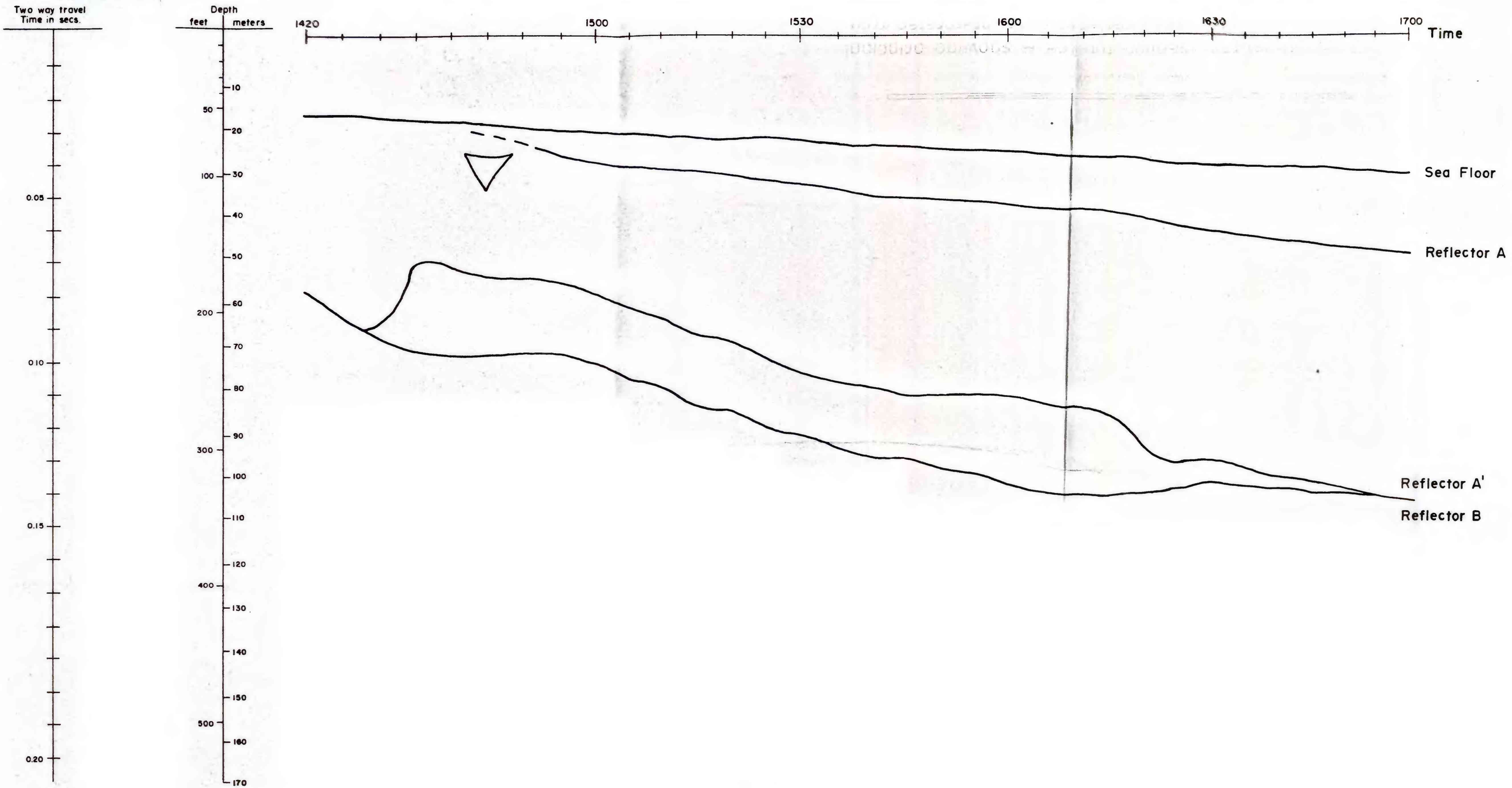
Figure 11-2 -- Cross section for line 2 showing principal sub-bottom reflectors as interpreted from seismic profile drawn to scale of figure 10.
