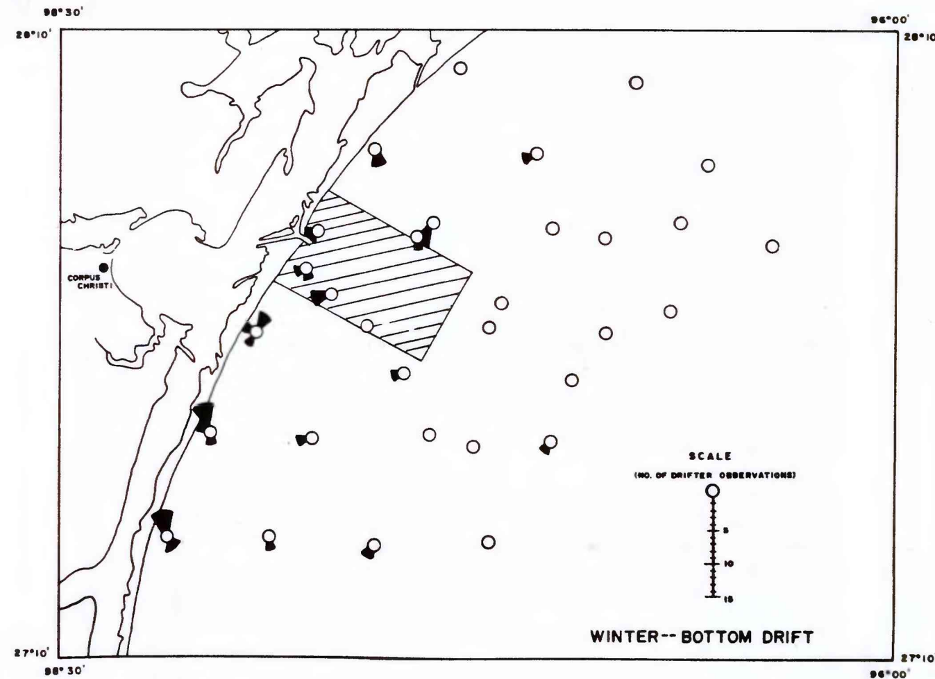
Figure 12B Fall/winter surface and bottom drift patterns along the south-central Texas coast
