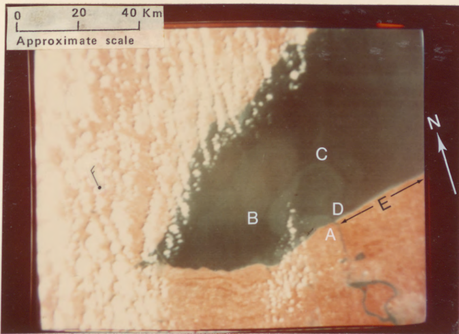
Figure 30. -- Part of LANDSAT-1 image 1353-15352, obtained July 11, 1973, showing the Niagara River (A), successive positions of its plume (B, C, D) and beach erosion (E) (photograph from Stanford Research Institute). EDC-010102.
