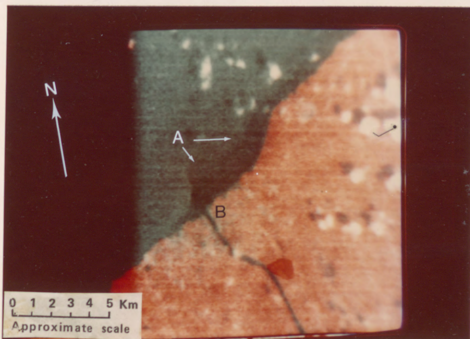
Figure 18. -- Part of LANDSAT-1 image 1386-15174, obtained Aug. 13, 1973, showing a clear water (dark) plume (A) at the mouth of the Oswego River (B) (photograph from Stanford Research Institute). EDC-010091.
