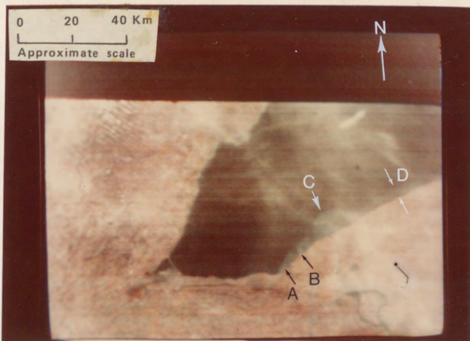
Figure 34. -- Part of LANDSAT-1 image 1497-15330, obtained Dec. 2, 1973, showing Port Dalhousie (A), the Welland Canal (B), Niagara River plume (C), and a beach erosion plume (D) (photograph from Stanford Research Institute). EDC-010106.
