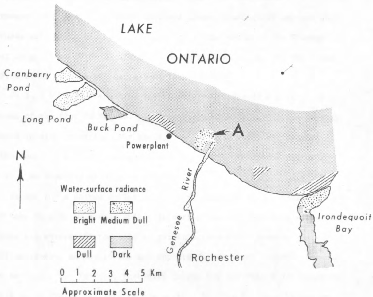
Figure 5. -- Genesee River plume as interpreted from aerial photographs obtained Aug. 20, 1972, at 1300 hours EST (photographs from NASA).
