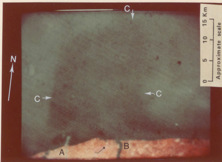
Figure 29. -- Part of LANDSAT-1 image 1407-15343, obtained Sept. 3, 1973, showing the Welland Canal (A), Niagara River (B), and the Niagara River plume (C) (photograph from Stanford Research Institute). EDC-010101.
