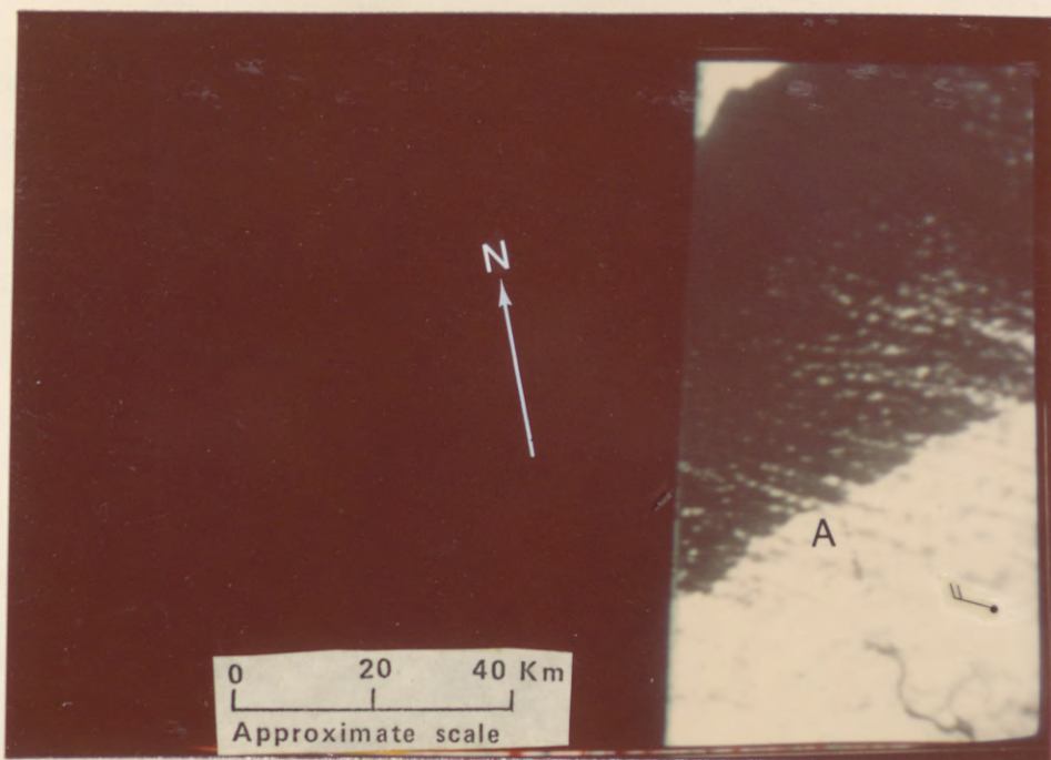
Figure 25. -- Part of LANDSAT-1 image 1568-15252, obtained Feb. 11, 1974, showing the Niagara River outlet (A) (photograph from Stanford Research Institute). EDC-010098.
