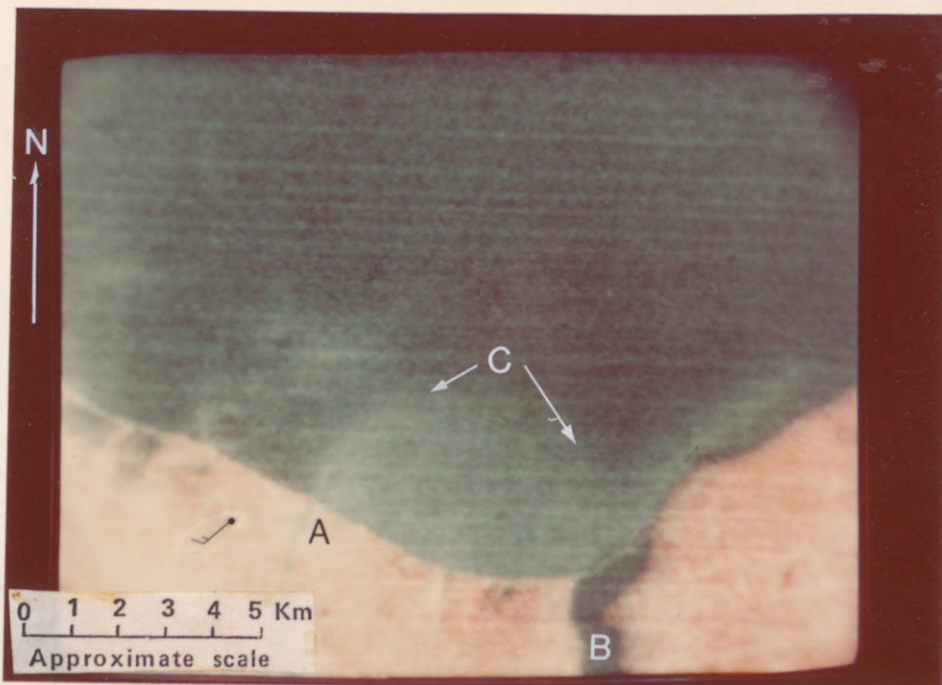
Figure 6. -- Part of LANDSAT-1 image 1297-15243, obtained May 16, 1973, showing the Genesee River outlet (A), Irondequoit Bay (B), and the Genesee River plume (C) (photograph from Stanford Research Institute). EDC-010079.
