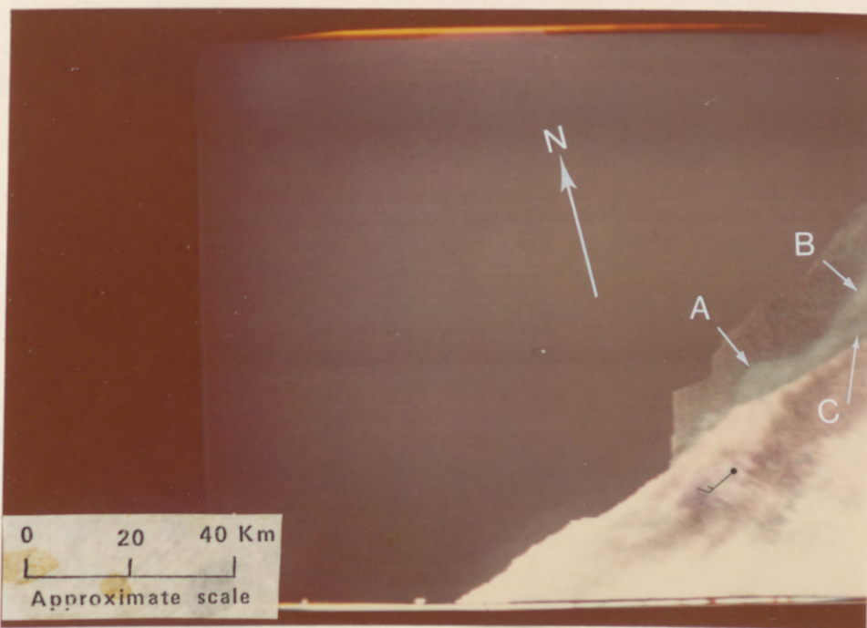
Figure 32. -- Part of LANDSAT-1 image 1551-15313, obtained Jan. 25, 1974, showing the Niagara River plume (A), its extension along the New York shore (C), and a cirrus cloud street (B) (photograph from Stanford Research Institute). EDC-010104.
