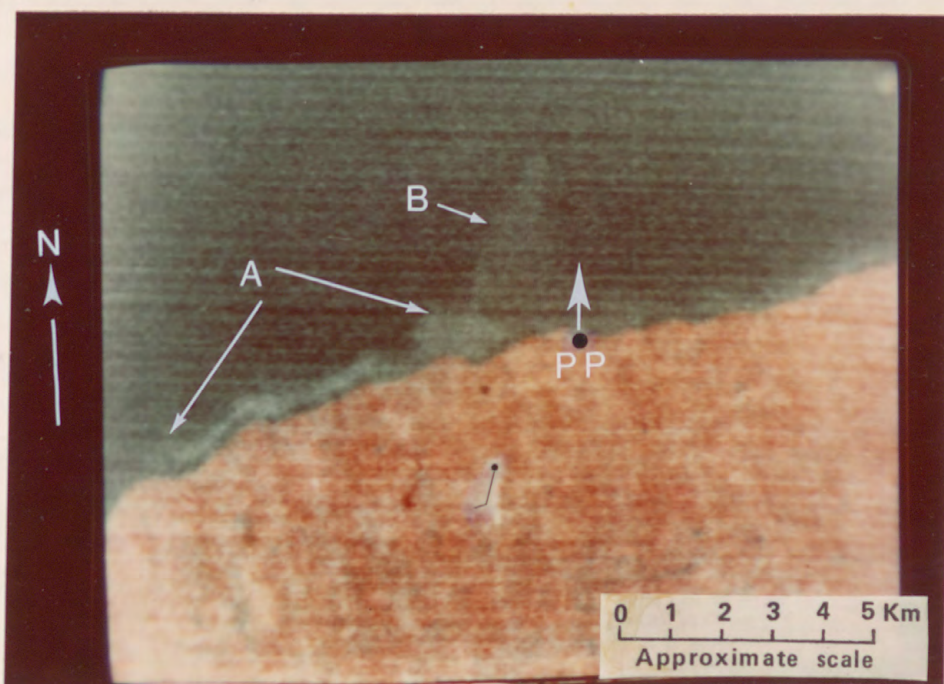
Figure 15. -- Part of LANDSAT-1 image 1423-15224, obtained Sept. 19, 1973, showing beach erosion plumes (A), and a plume (B) created by discharge from the Ginna powerplant (PP) (photograph from Stanford Research Institute). EDC-010088.
