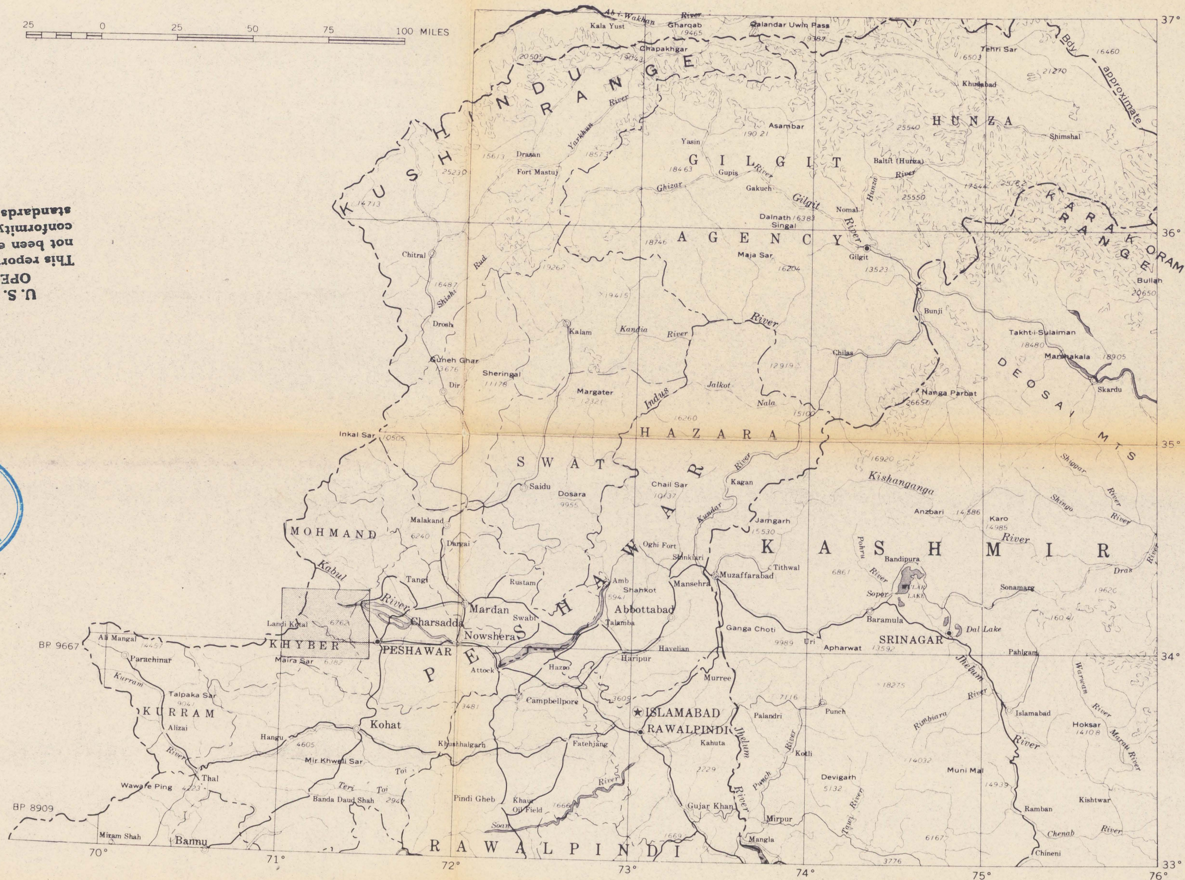
Figure 1—Index map showing location of the Khyber Pass area, Pakistan
