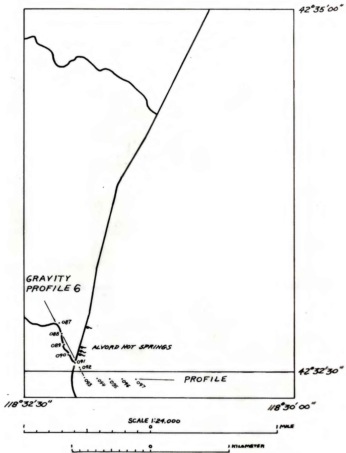
GRAVITY PROFILE AT ALVORD HOT SPRINGS, OREGON
