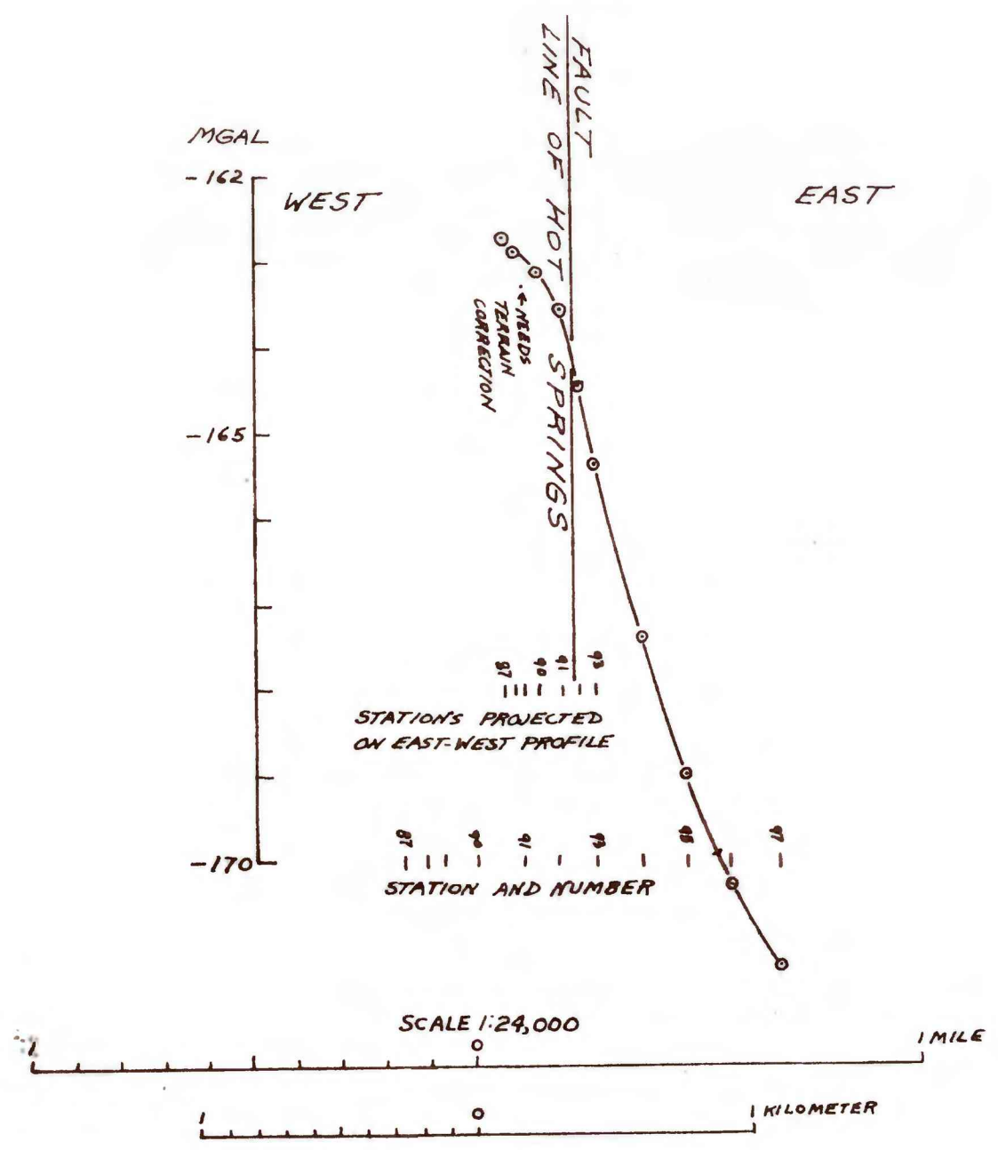
GRAVITY PROFILE AT ALVORD HOT SPRINGS, OREGON (PROFILE 6)
