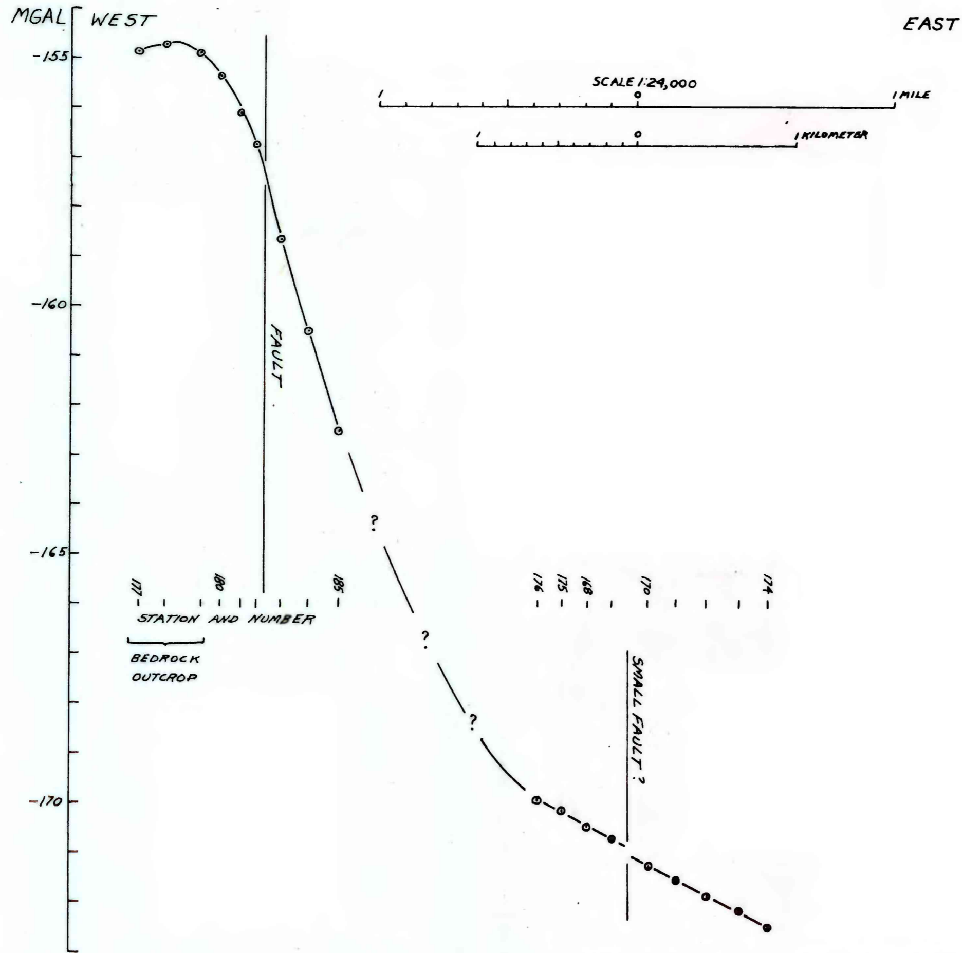
GRAVITY PROFILE IN THE ANDREWS QUADRANGLE, OREGON (PROFILE 7)
