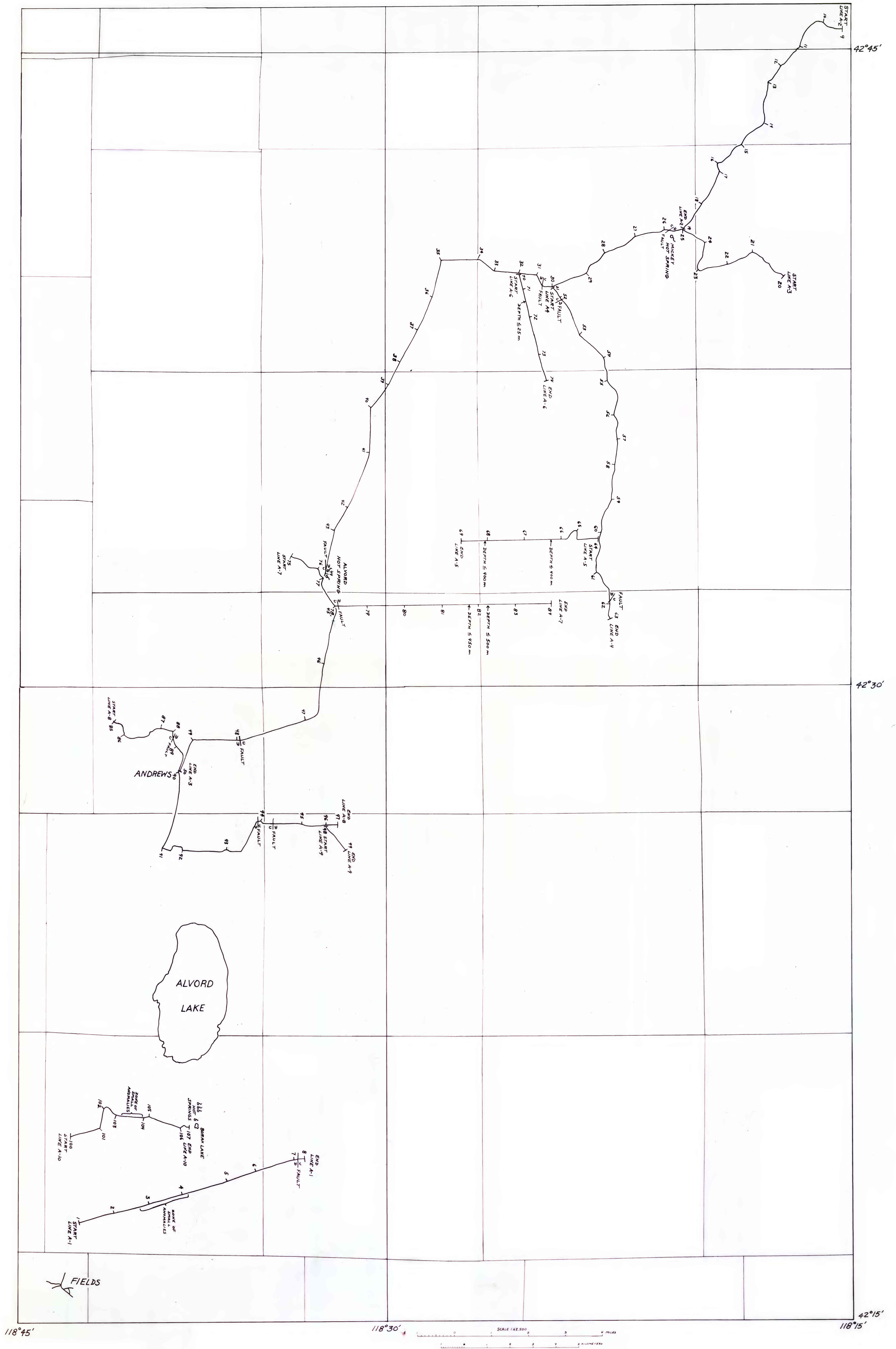
LOCATION AND INTERPRETATION OF TRUCK-MOUNTED MAGNETOMETER TRAVERSES, ALVORD DESERT AREA, OREGON
