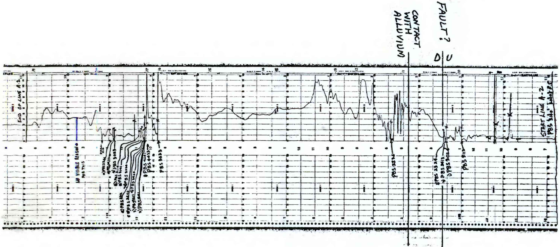
MAGNETIC PROFILE A-2
