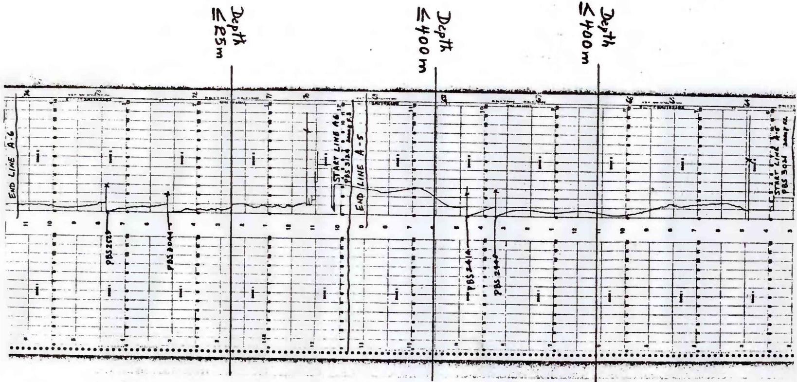
MAGNETIC PROFILES A-5 and A-6
