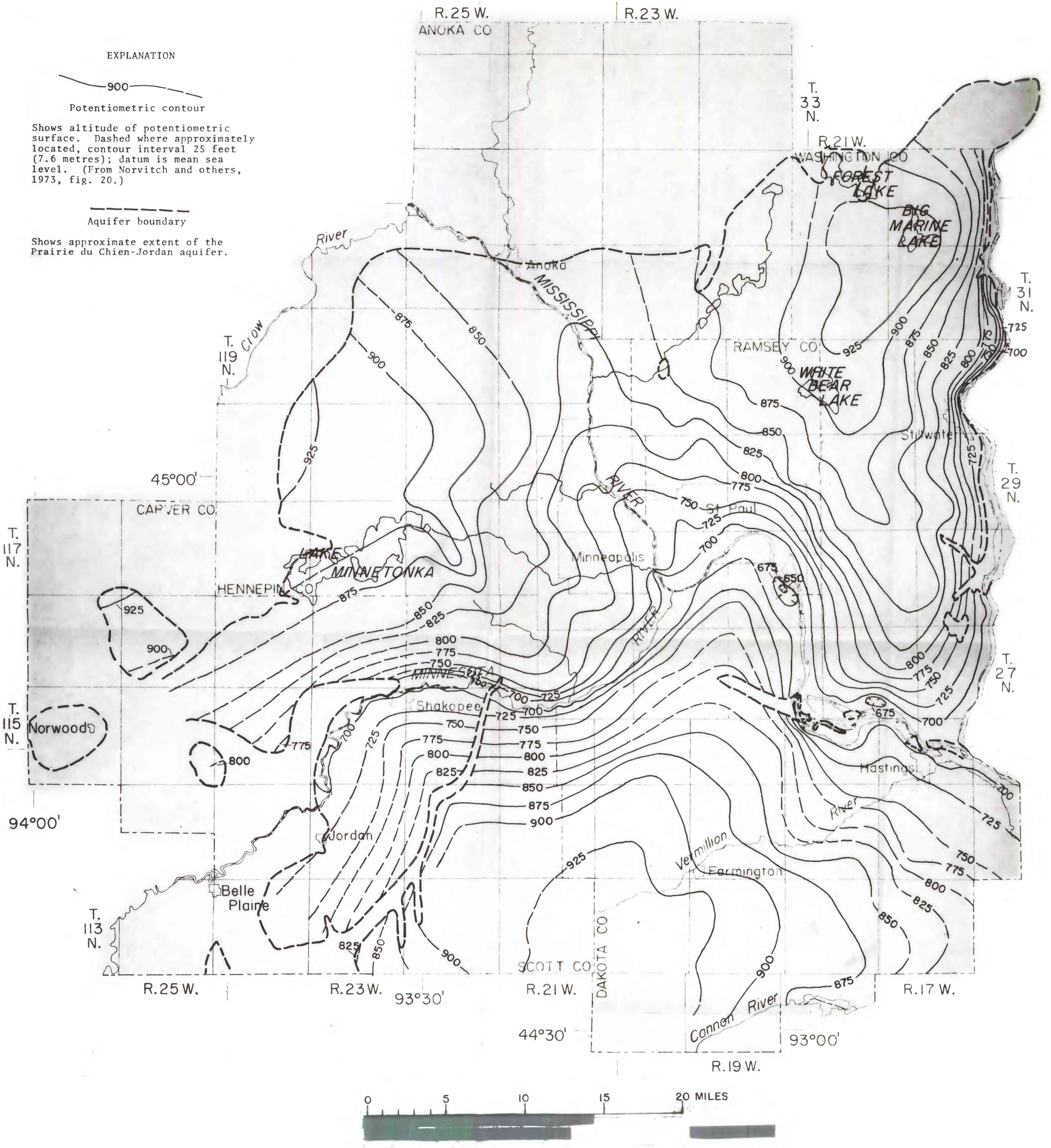
21 Potentiometric surface in the Prairie du Chien - Jordan aquifer, winter 1970-71.
