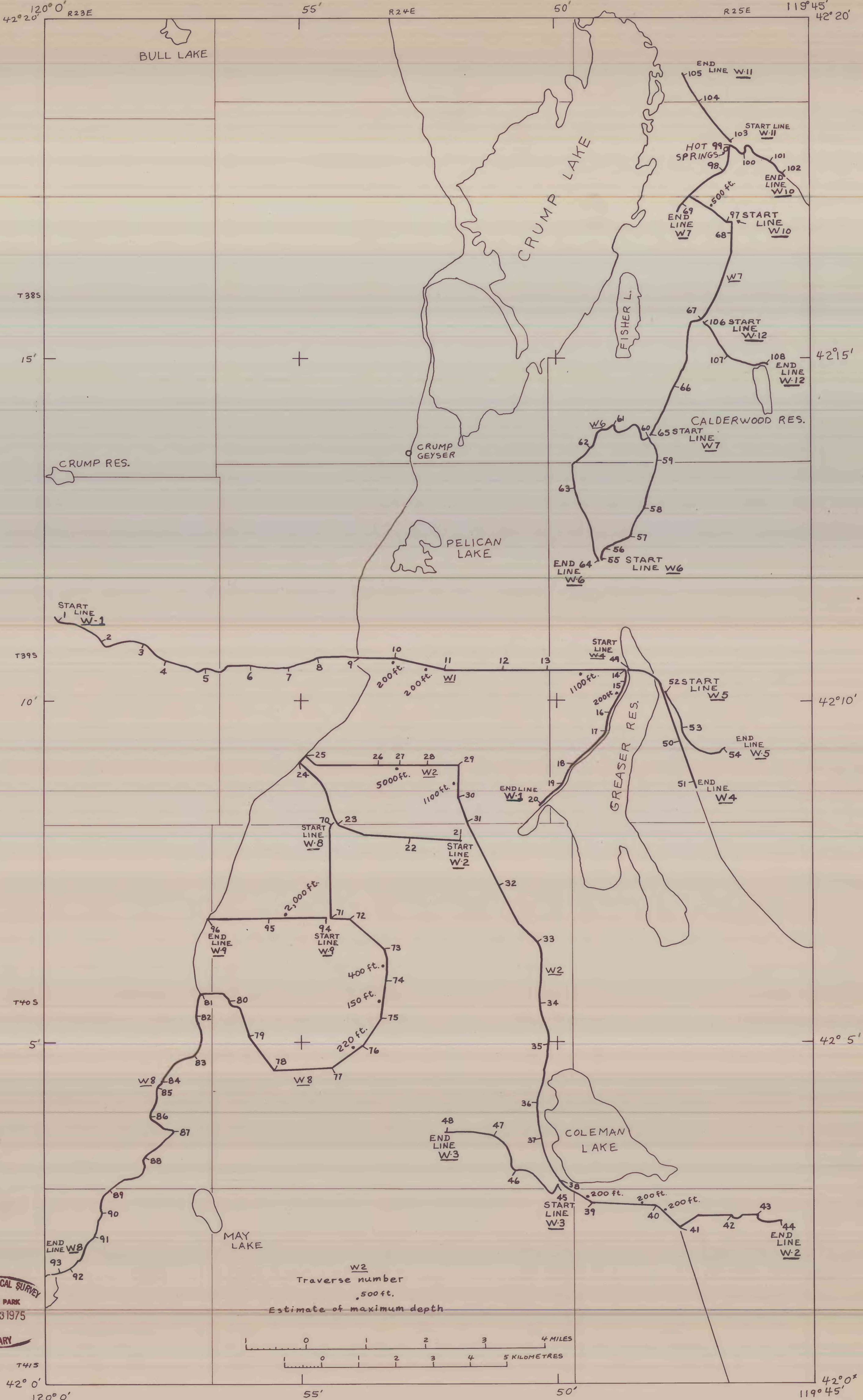
LOCATION OF TRUCKBORNE MAGNETOMETER TRAVERSES
