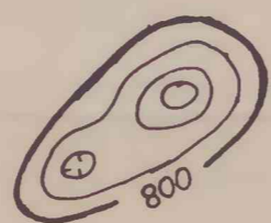
Magnetic contours
