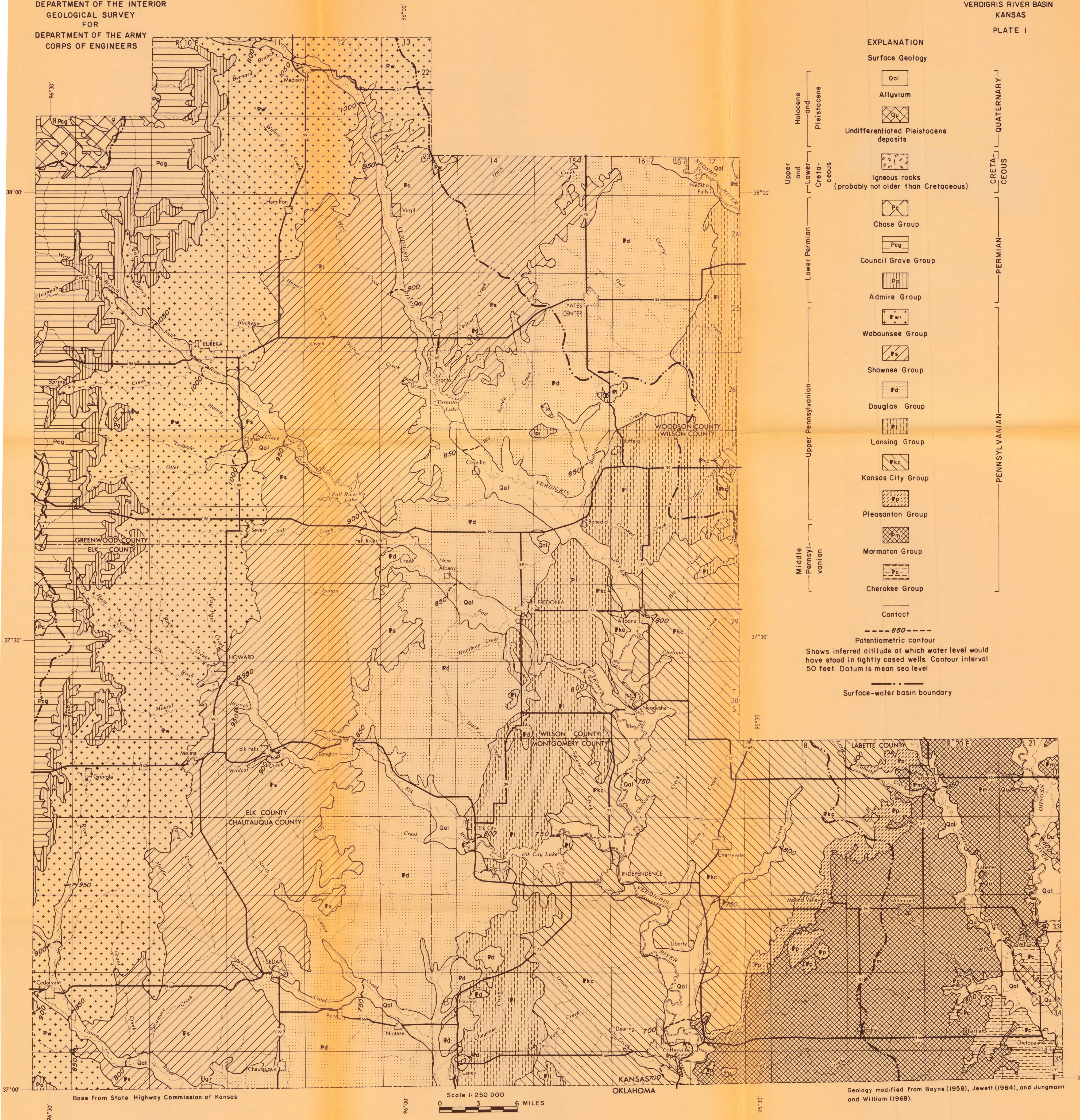
GEOLOGIC MAP SHOWING CONFIGURATION OF POTENTIOMETRIC SURFACE
