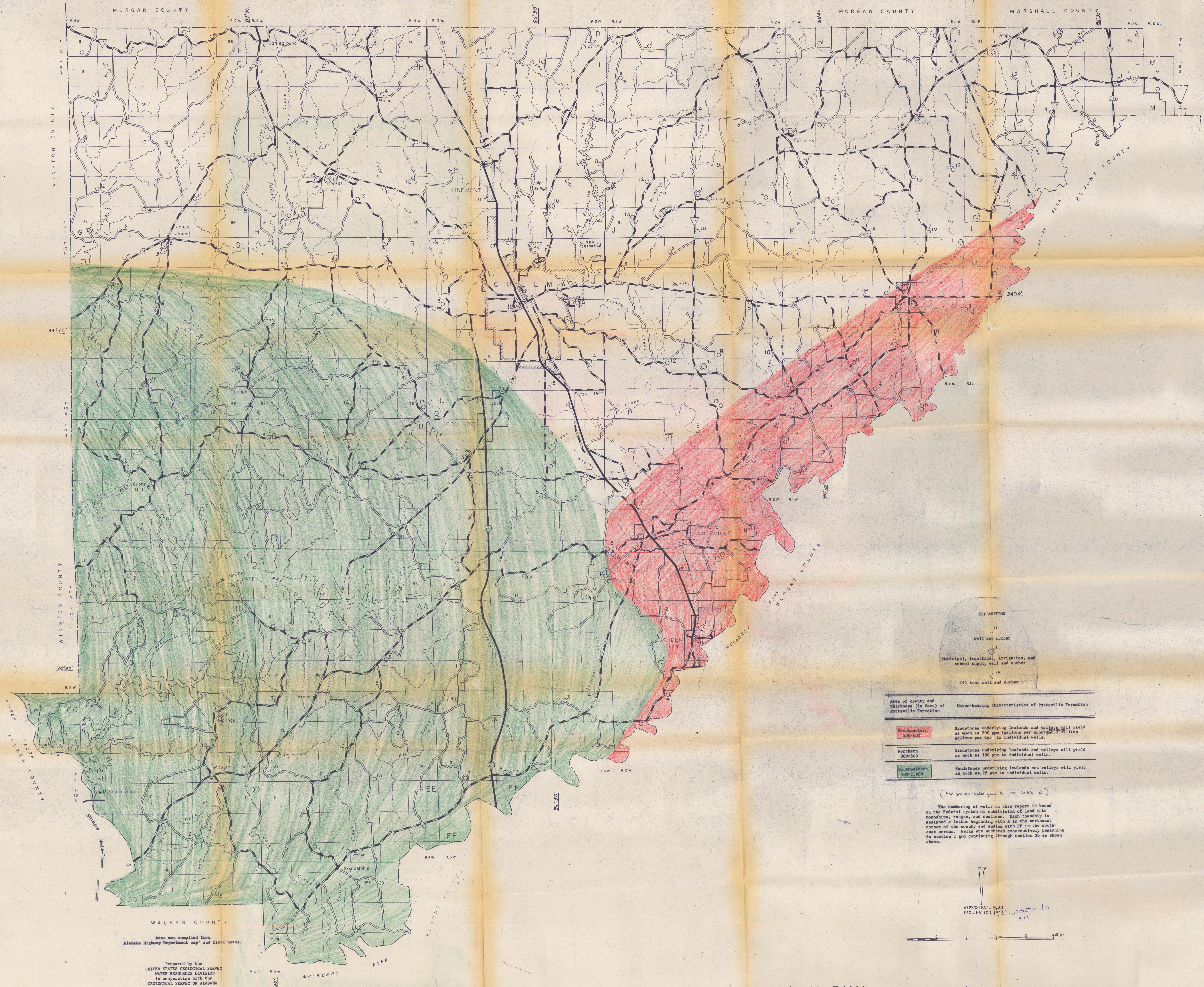
FIGURE 3 --AVAILABILITY OF GROUND WATER IN CULLMAN COUNTY, ALABAMA (by Robert J Faust -1970)
