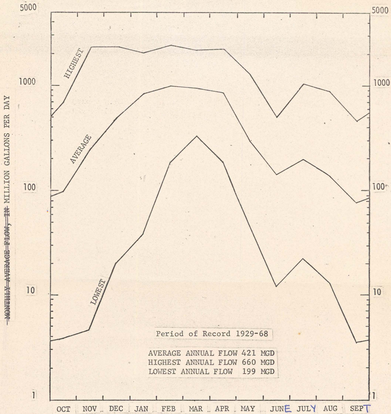
Figure 5.--Hydrograph of average monthly flows of Mulberry Fork near Garden City, Alabama.
