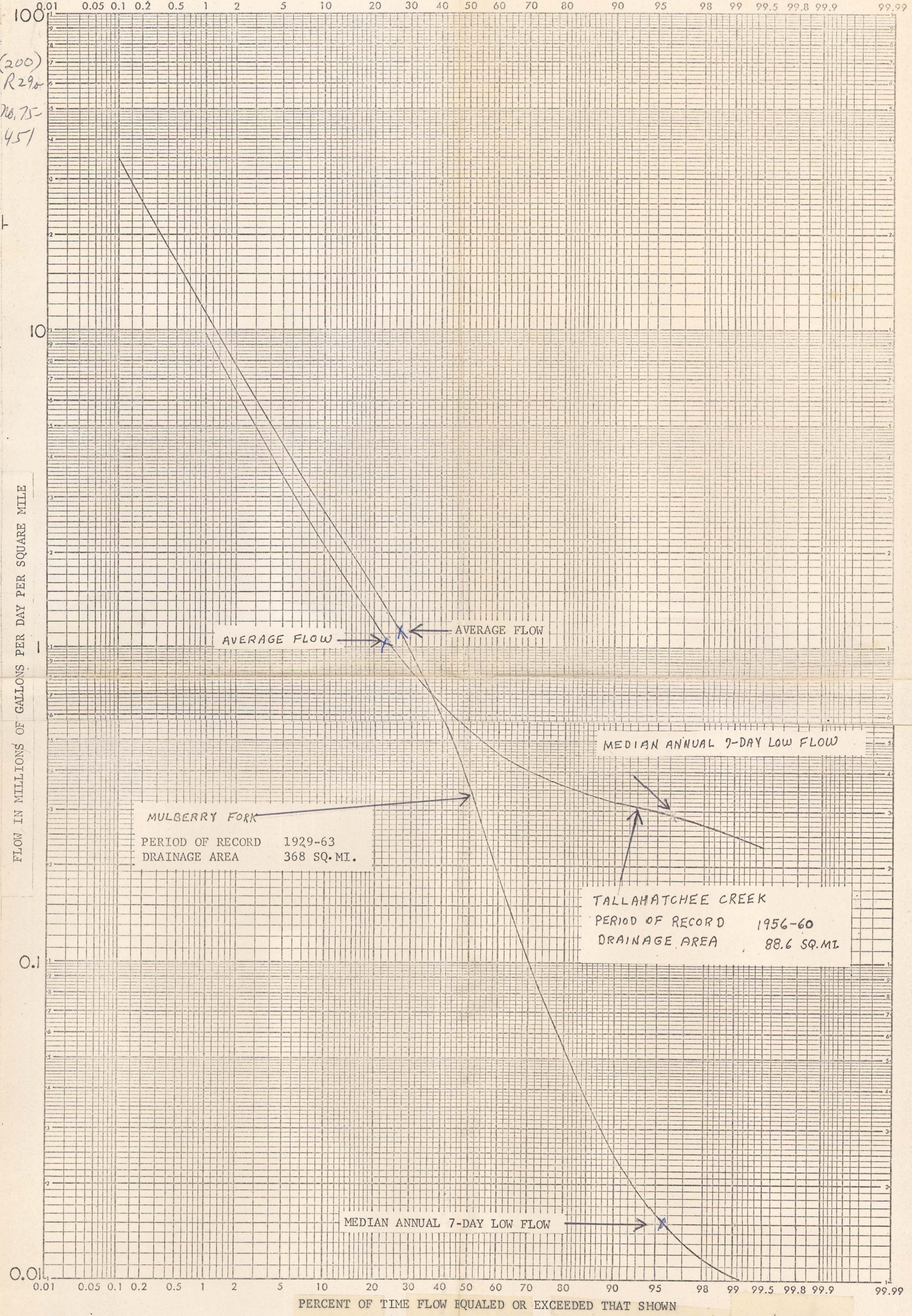
Figure 6.5--Flow duration curves for Mulberry Fork near Garden City and Tallahatchee Creek near Wellington, Ala.
