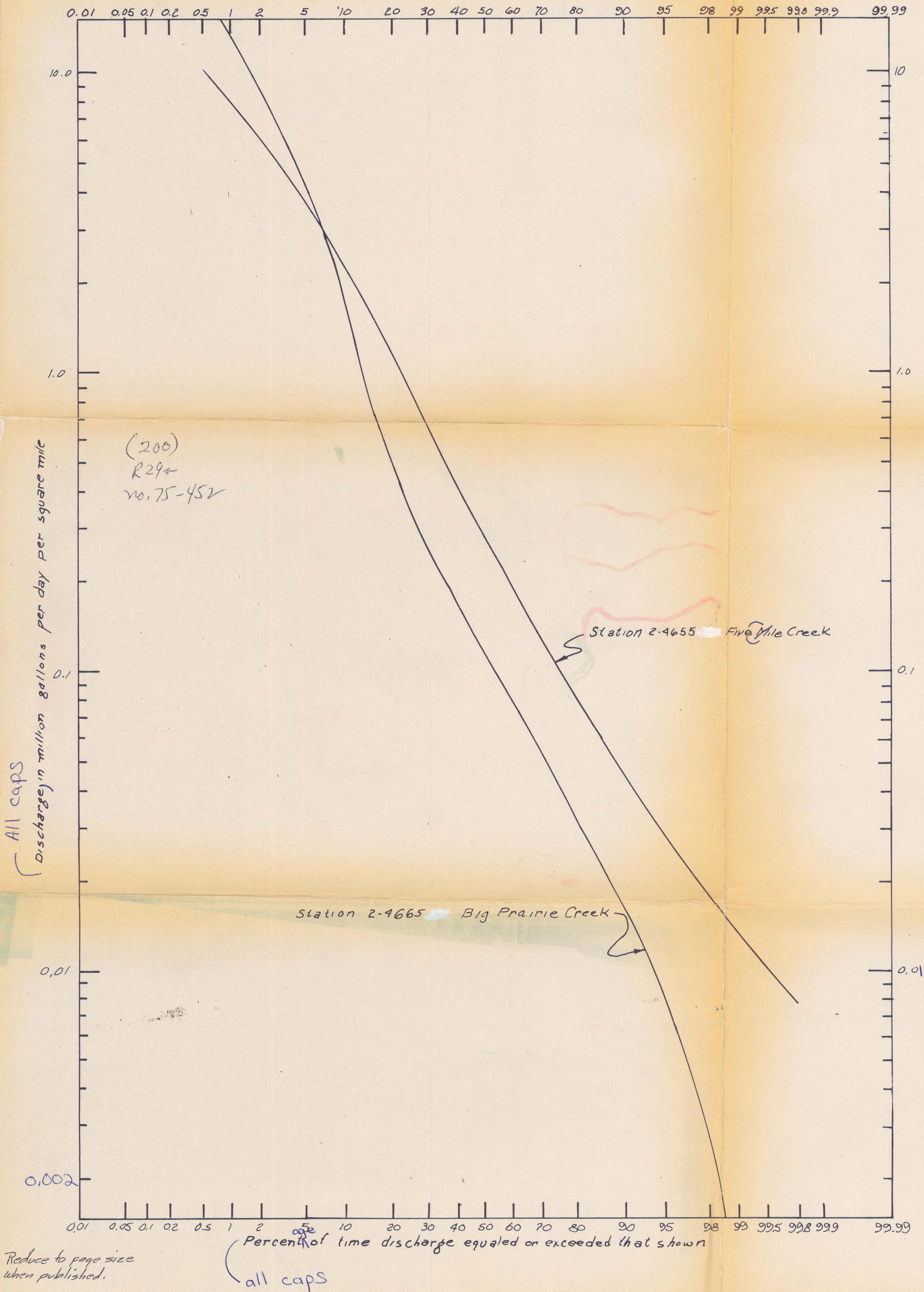
FIGURE 7-FLOW-DURATION CURVES FOR TWO STREAMS IN HALE COUNTY FOR PERIOD 1940-56
