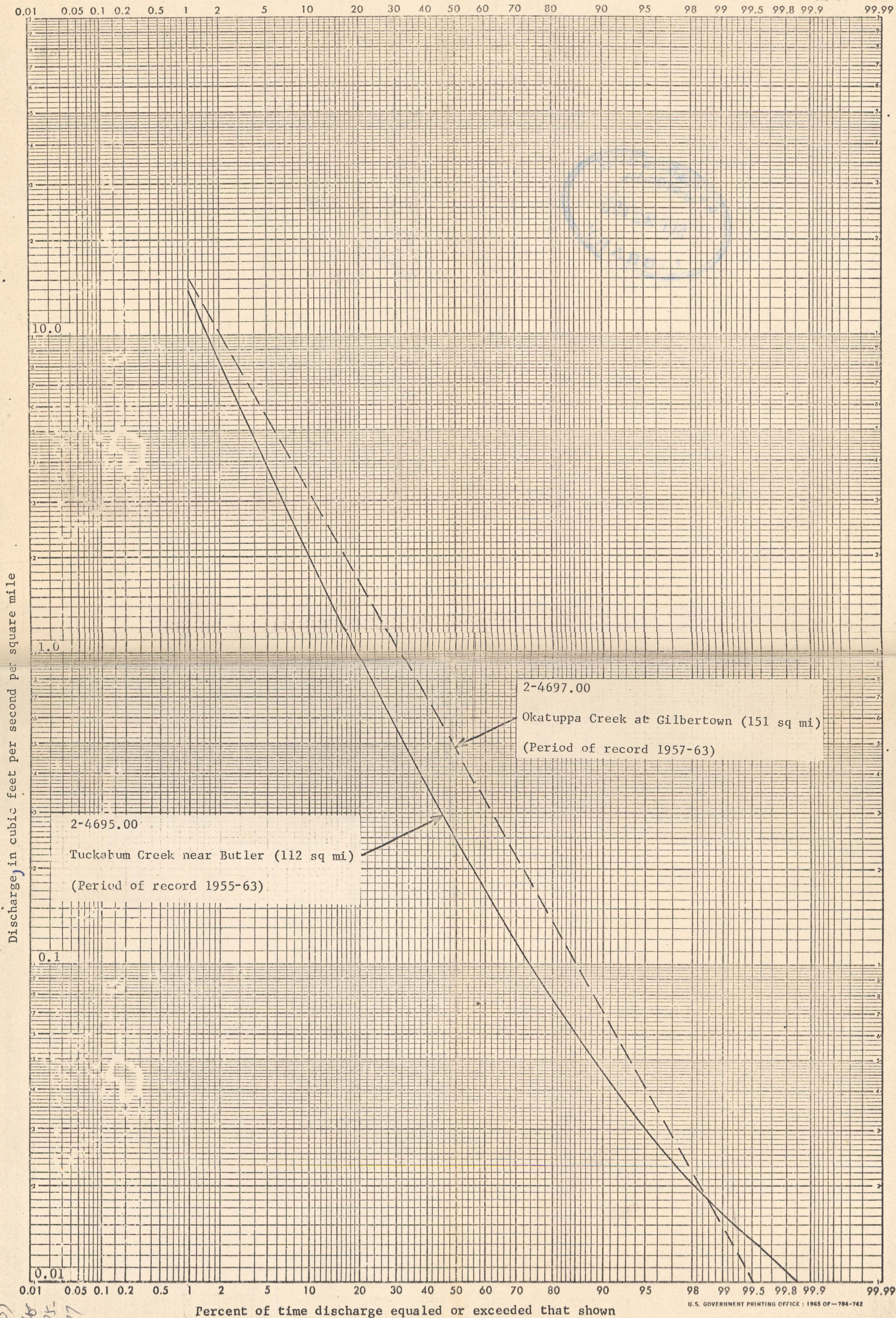
Figure 5.--Flow-duration curves for creeks in Choctaw County.
