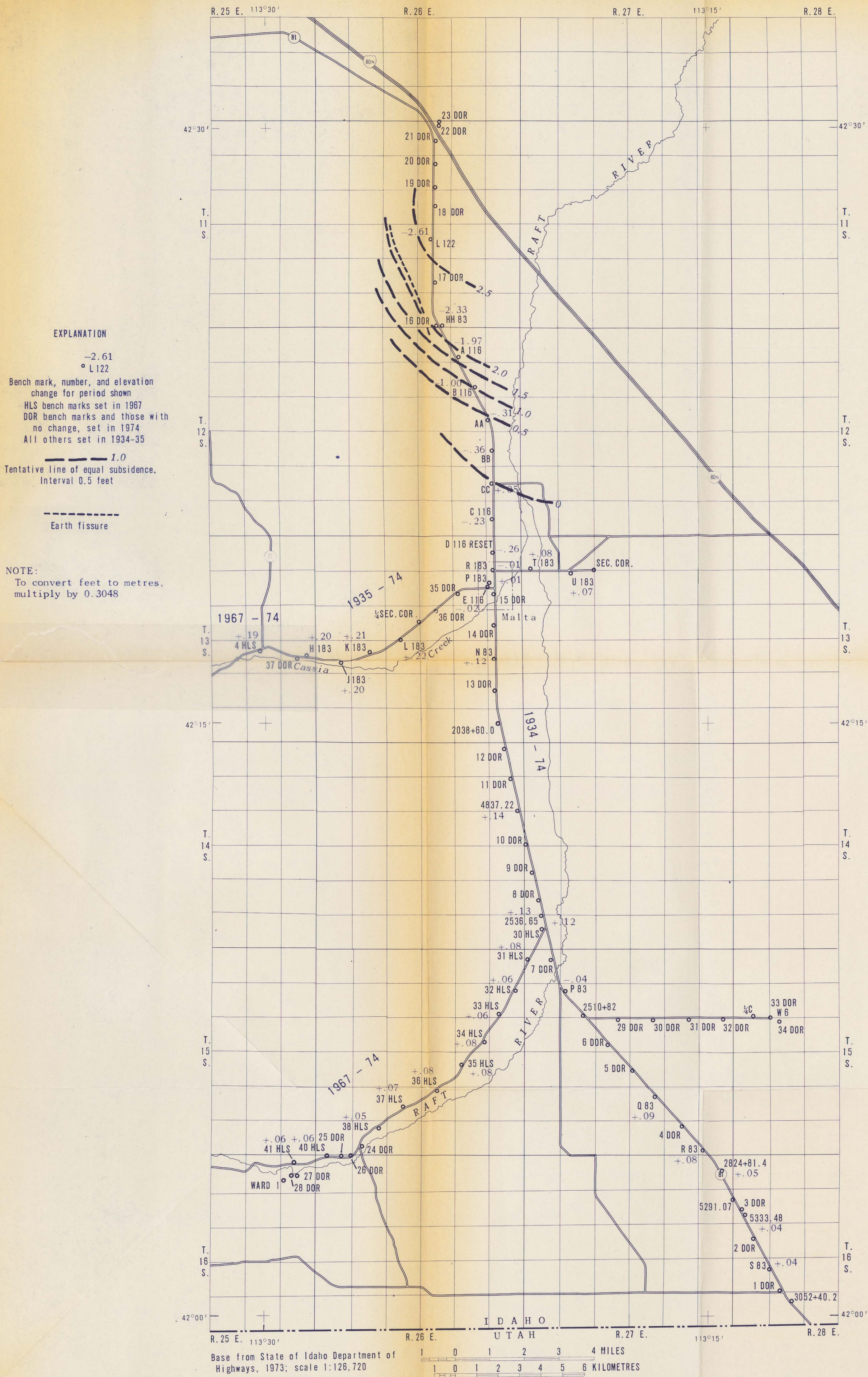
FIGURE 2.—Measured change in elevation of bench marks, Raft River Valley, Idaho
