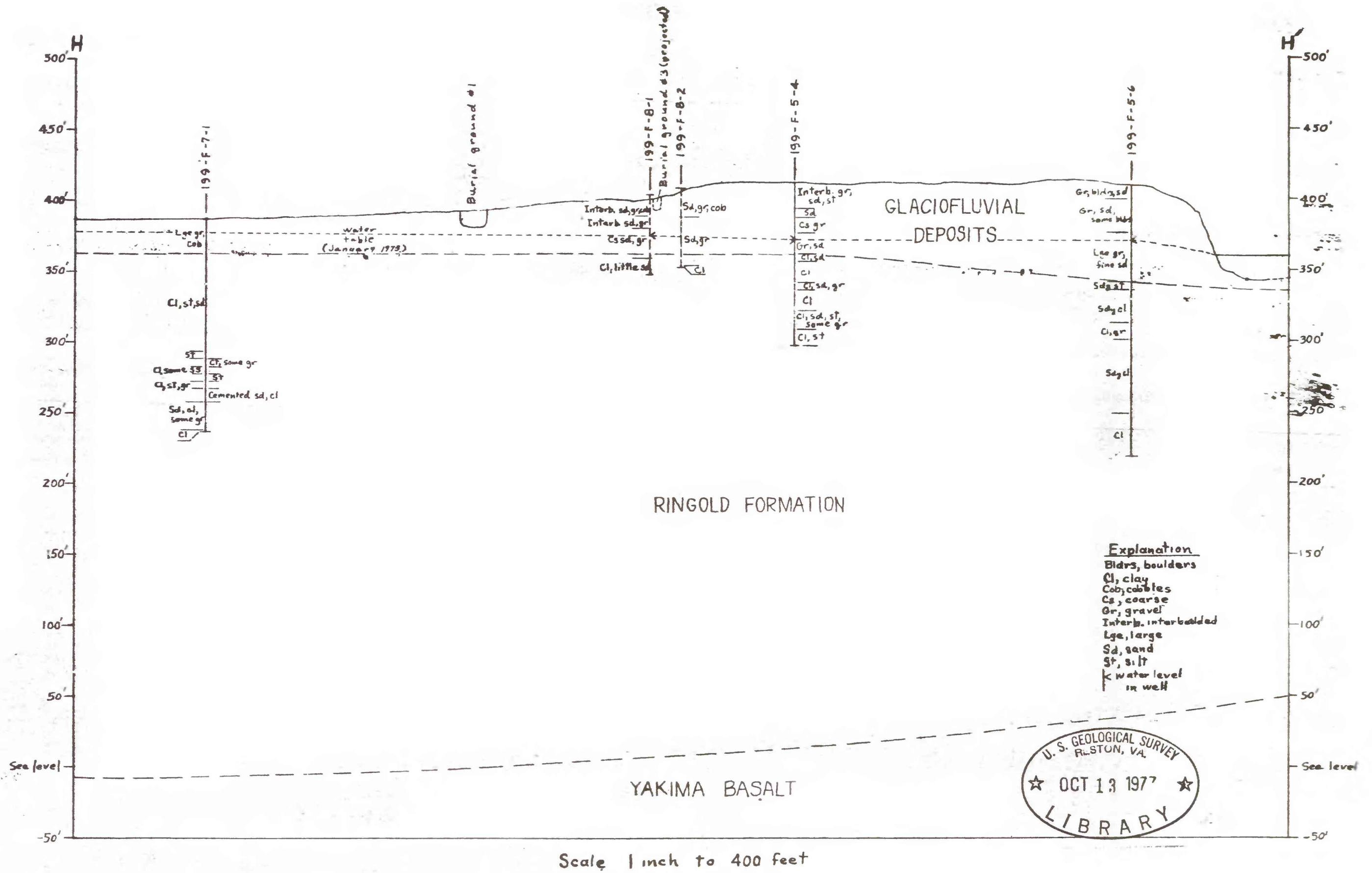
Figure 19.-- Geologic section H-H' across the 100 F Area.
