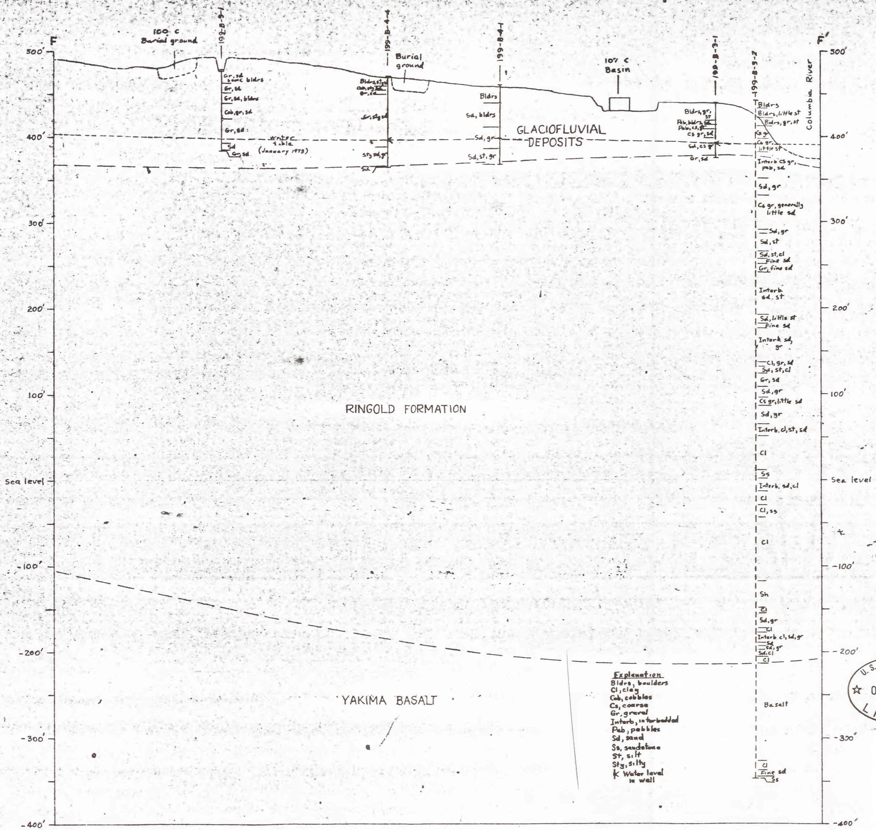
Figure 13.-- Geologic section F-F' across the 100 B Area.
