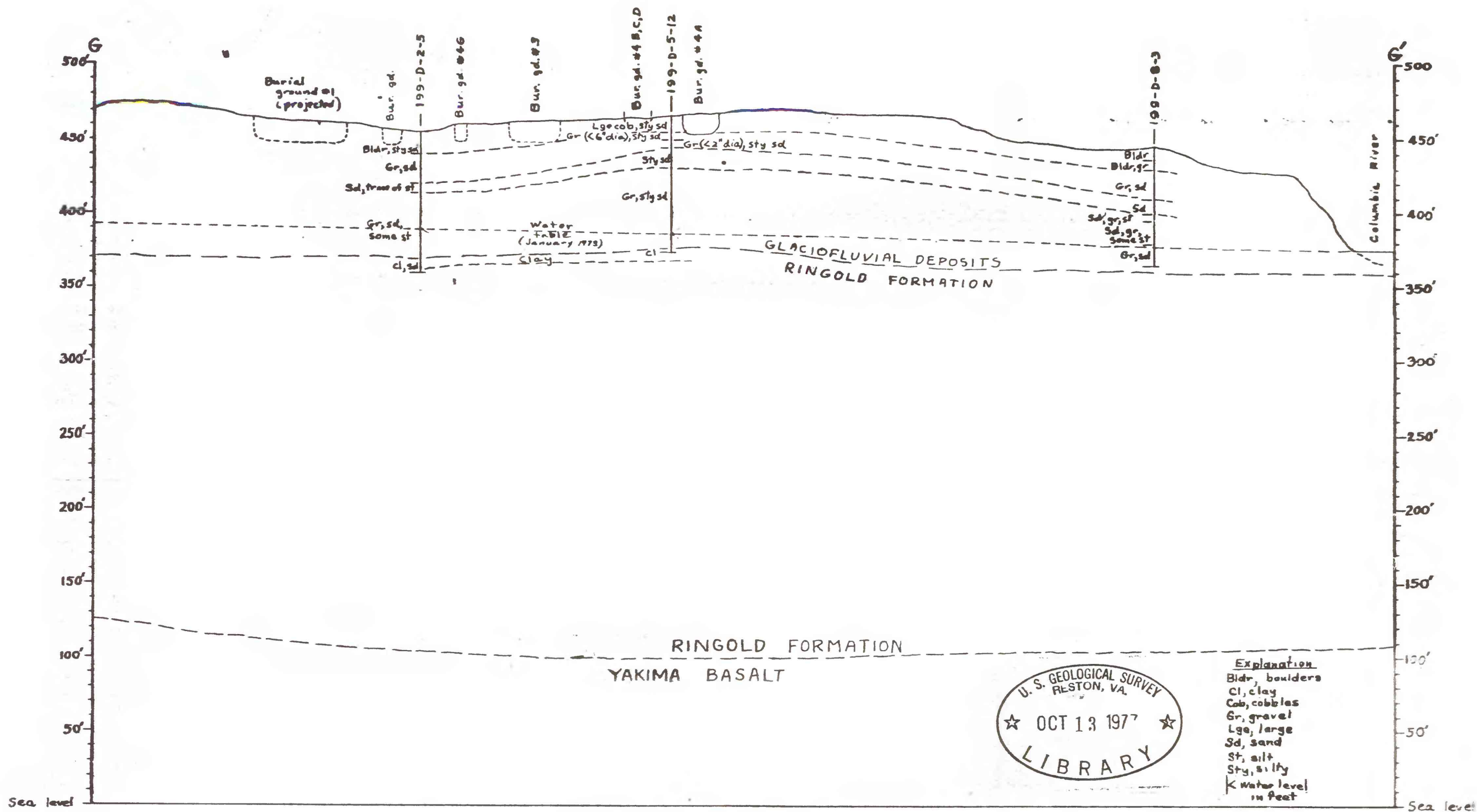
Figure 16.-- Geologic section G-G' across the 100 D Area.
