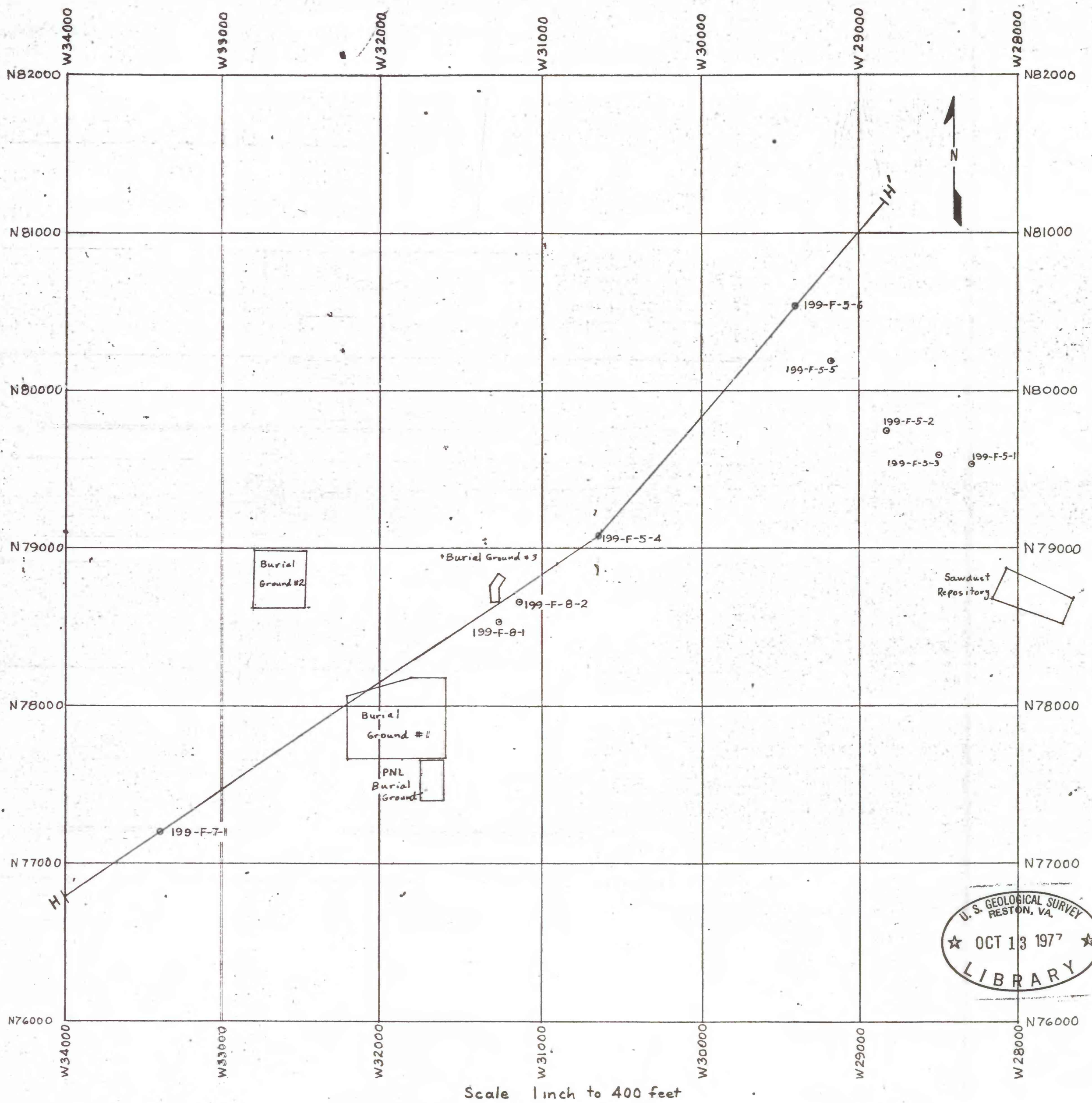
Figure 18.-- Plan view showing line of section H-H' and nearby wells and burial grounds.
