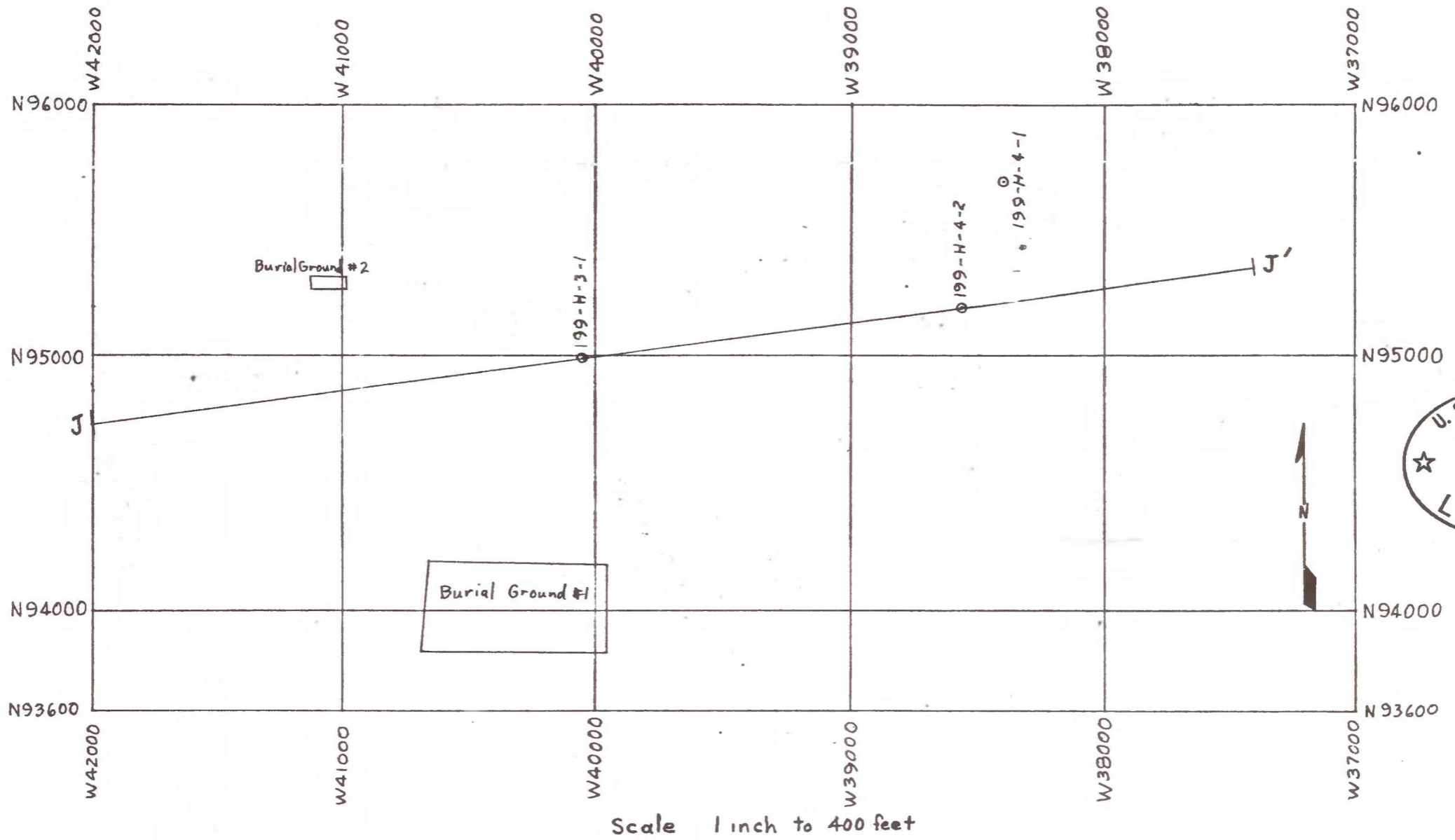
Figure 21.--Plan view showing line of section J-J' and nearby wells and burial grounds.
