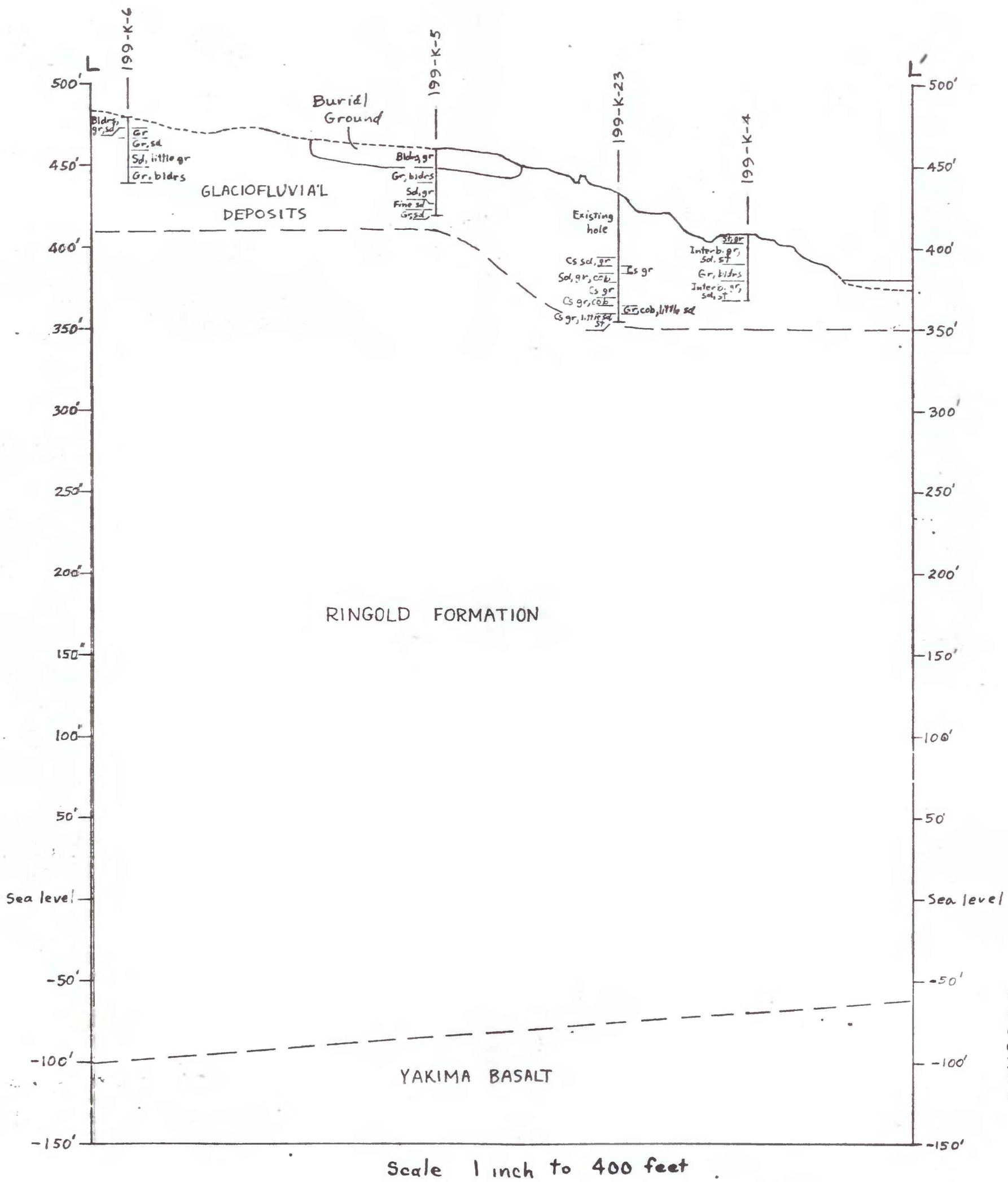
Figure 26.-- Geologic section L-L' across the 100 K Area.
