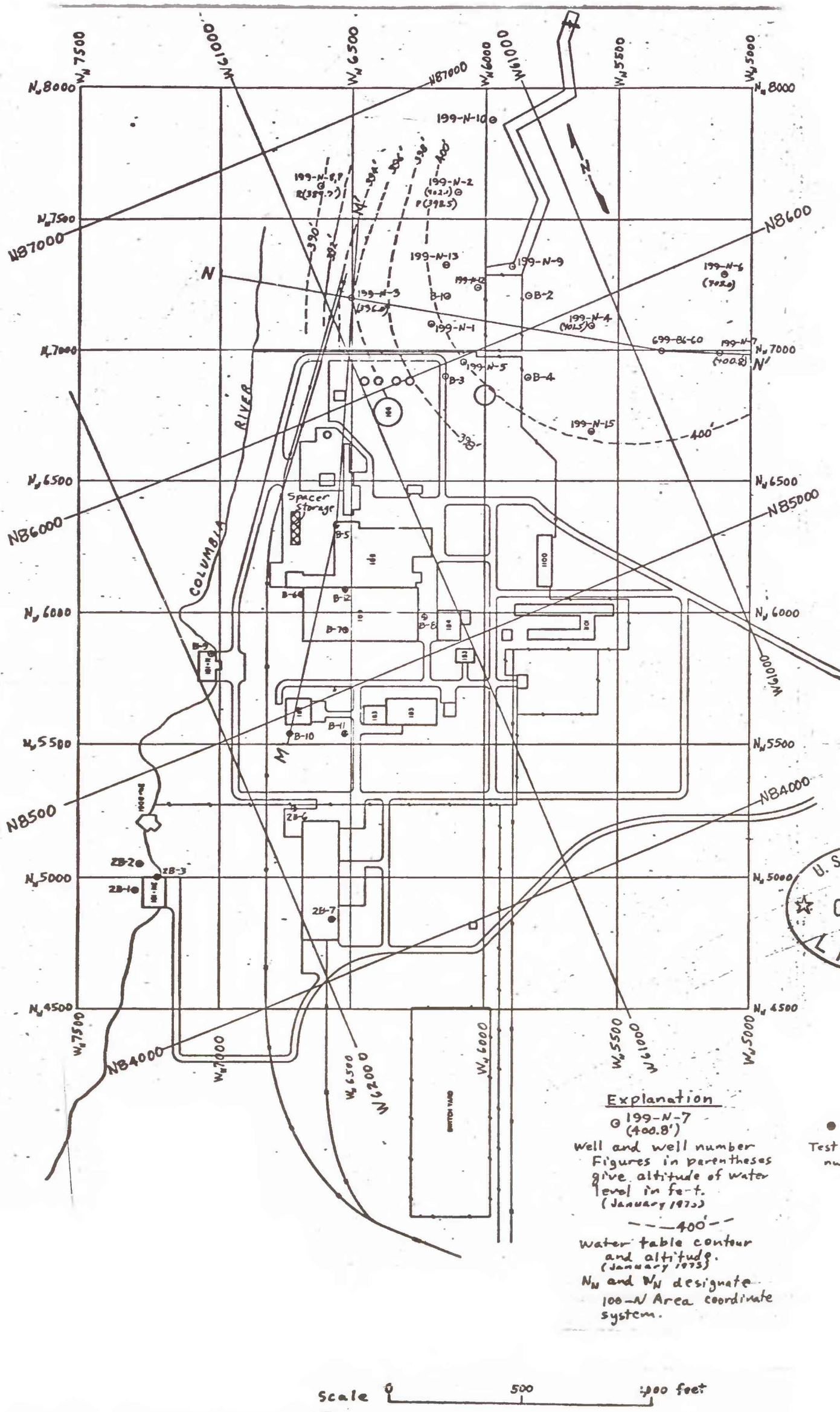
Figure 27.-- Map of the 100 N Area showing the spacer-storage structure wells and test borings, and lines of sections M-M' and N-N'.
