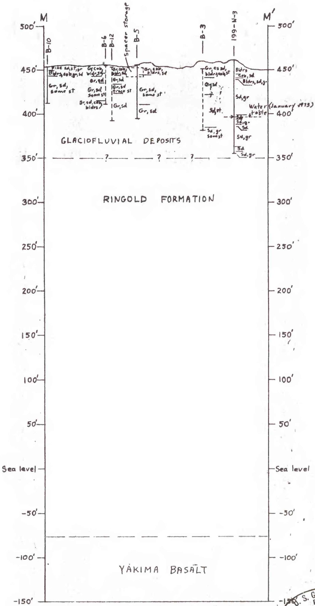
Figure 29.-- Geologic section M-M' across the 100 N Area.
