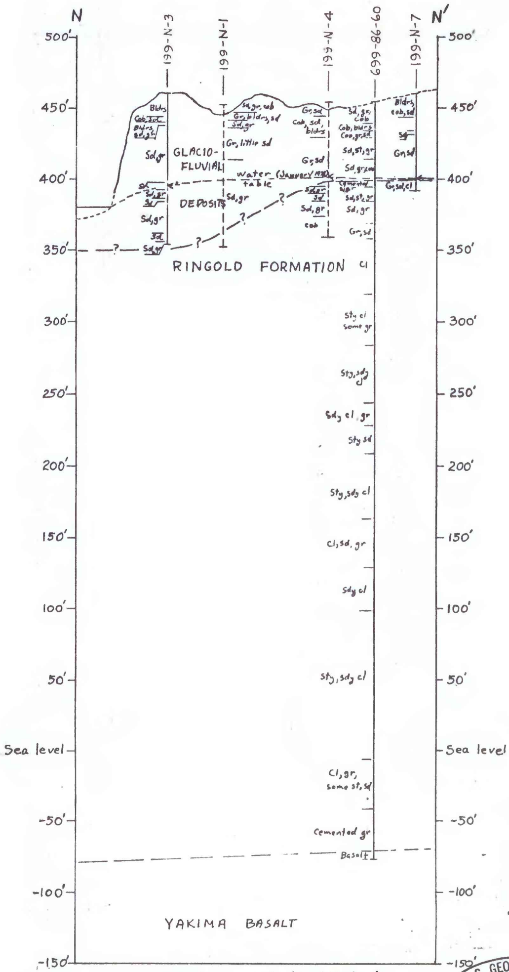
Figure 30.- Geologic section N-N' across the 100 N Area.
