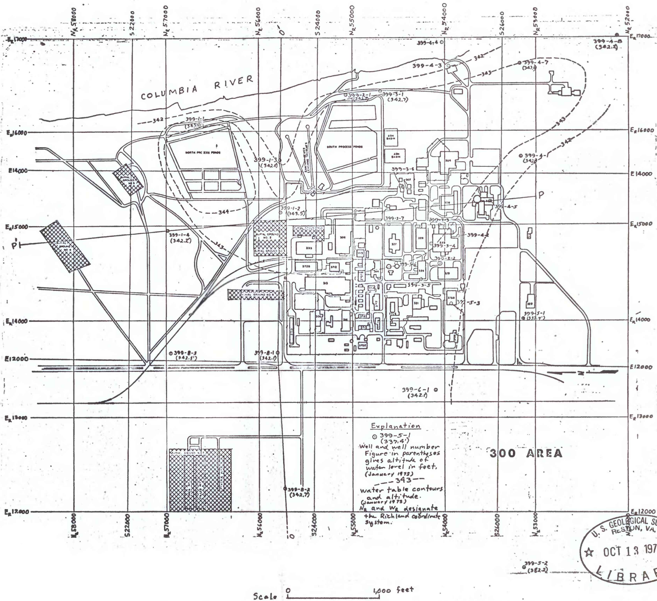
Figure 31.-- Map of the 300 Area showing burial grounds, monitoring and test wells and lines of sections 0-0' and P-P'
