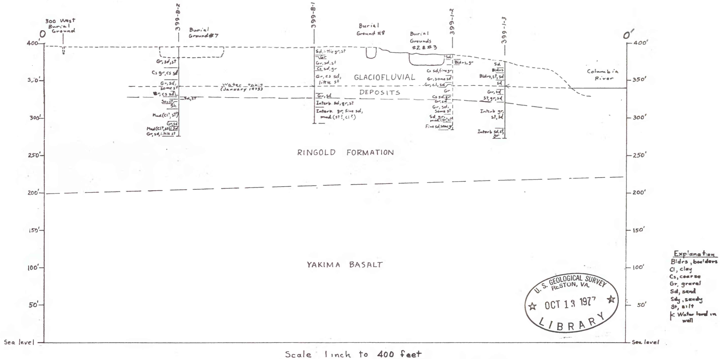
Figure 33.-- Geologic section 0-0' across the 300 Area.
