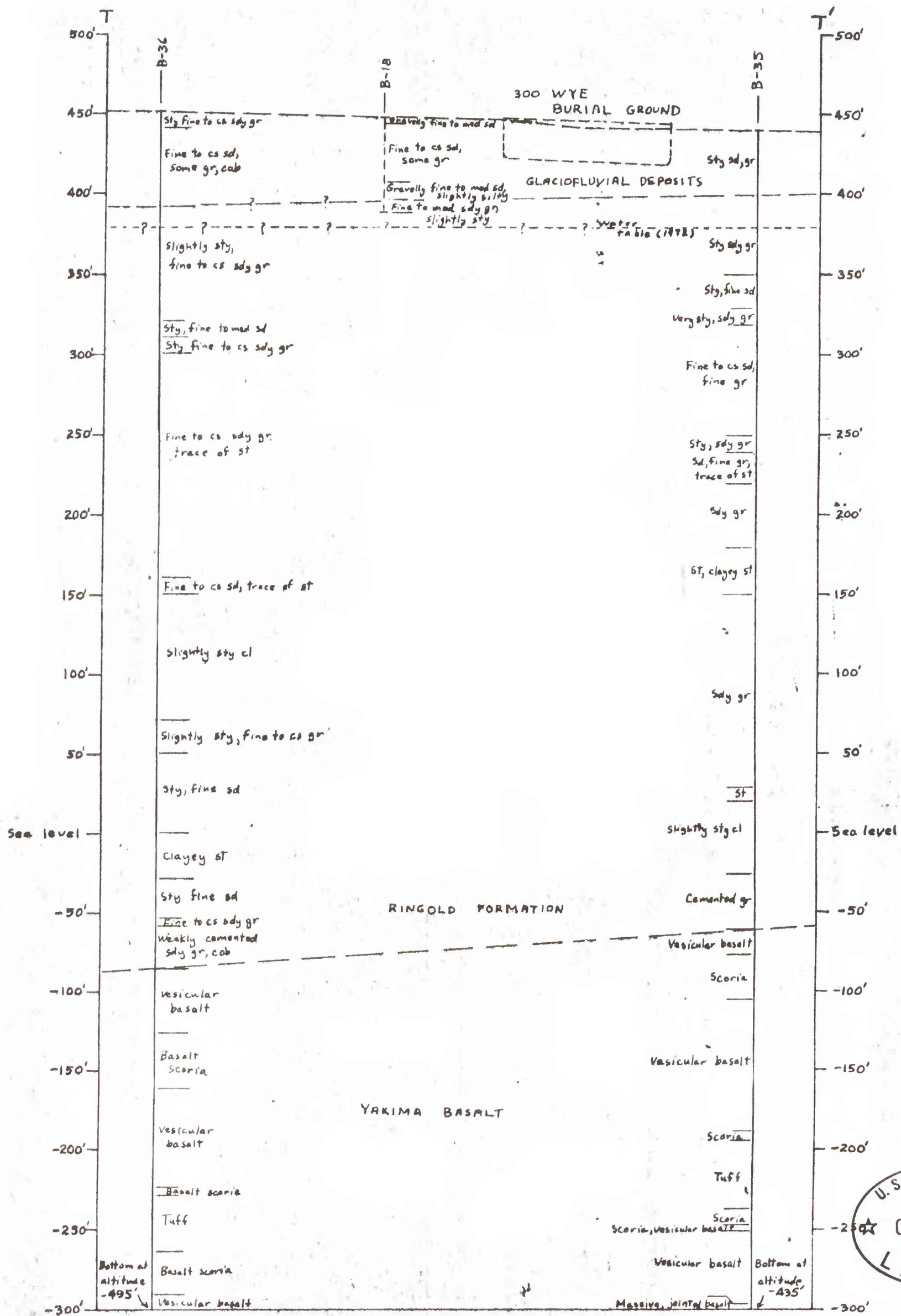
Scale 1 inch to 400 feet Figure 39.-- Geologic section T-T'
