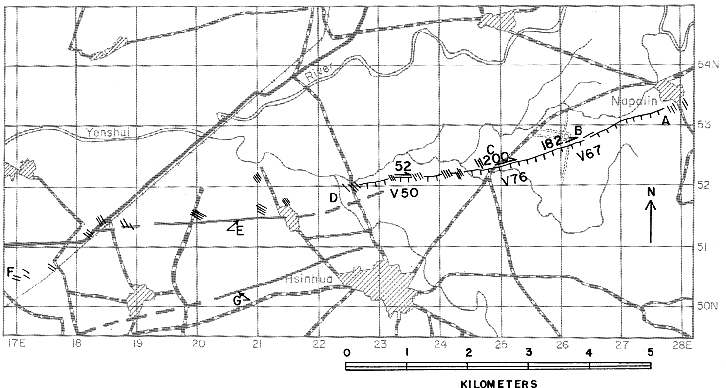
Figure 7. Map showing 1946 fault trace, after Chang, Chow, and Chen (1947). Displacements given in centimeters; V indicates vertical displacements; barbs on downthrown side. Faults E and G shown on screened base are from Sun (1964, pl. 3).
