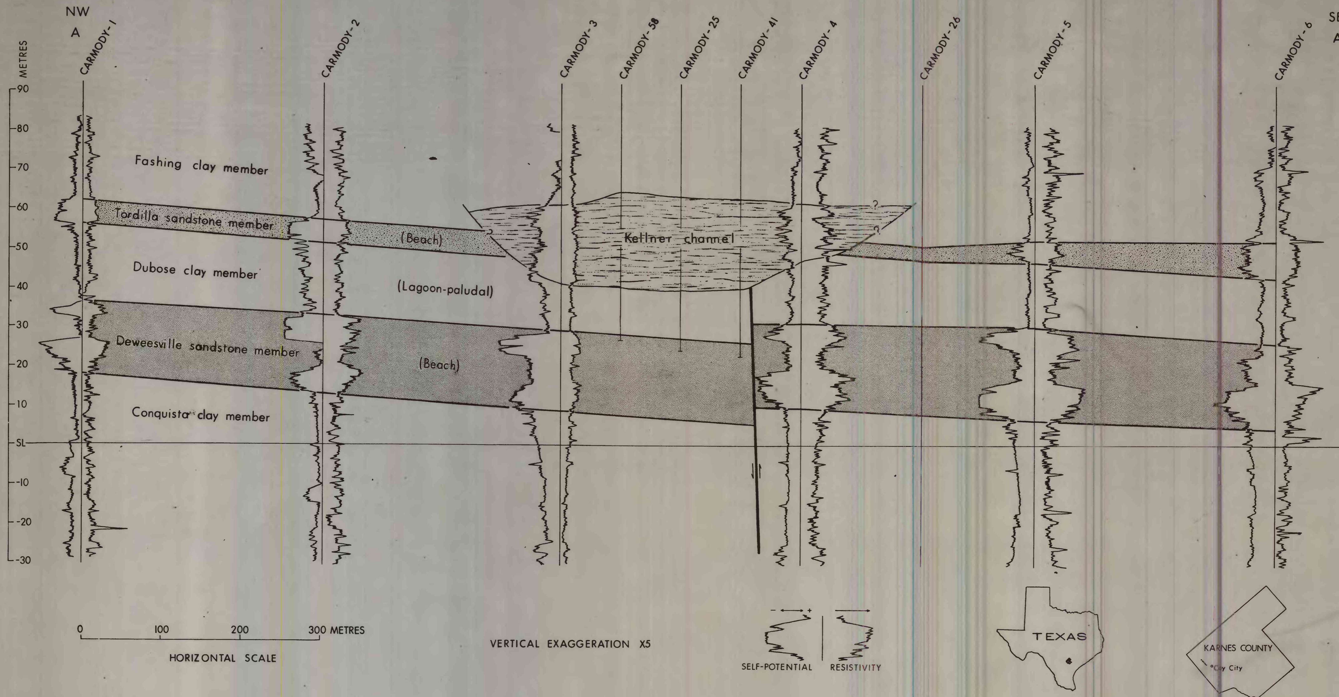
PLATE 2.--ELECTRIC-LOG SECTION ACROSS ROSENBRICK URANIUM DEPOSIT (PROFILE A-A', FIG. 3). DEPOSIT IS IN KELLNER CHANNEL OF FASHING CLAY MEMBER ERODED INTO TORDILLA SANDSTONE AND DUBOSE CLAY MEMBERS OF WHITSETT FORMATION. By Kendell A. Dickinson, 1976.
