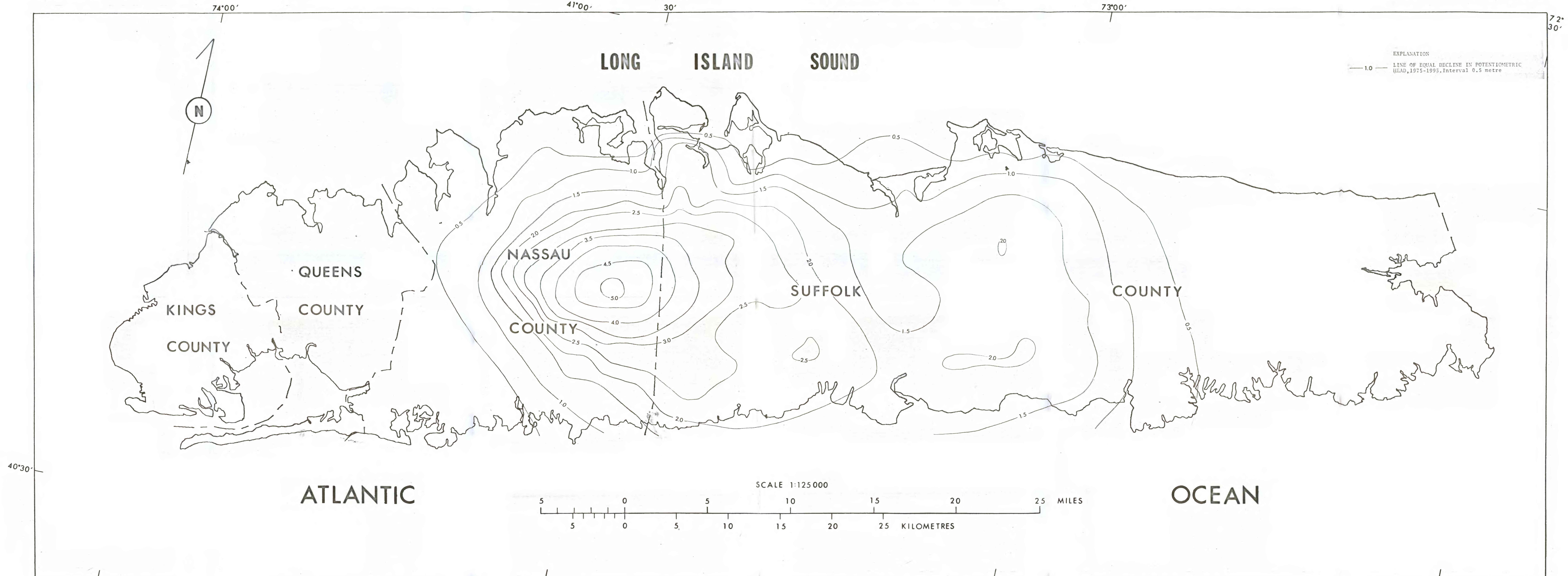
Figure 5.--Estimated head decline in Magothy aquifer resulting from proposed sewer construction in Nassau and Suffolk Counties, Long Island, New York from 1975 to 1995.
