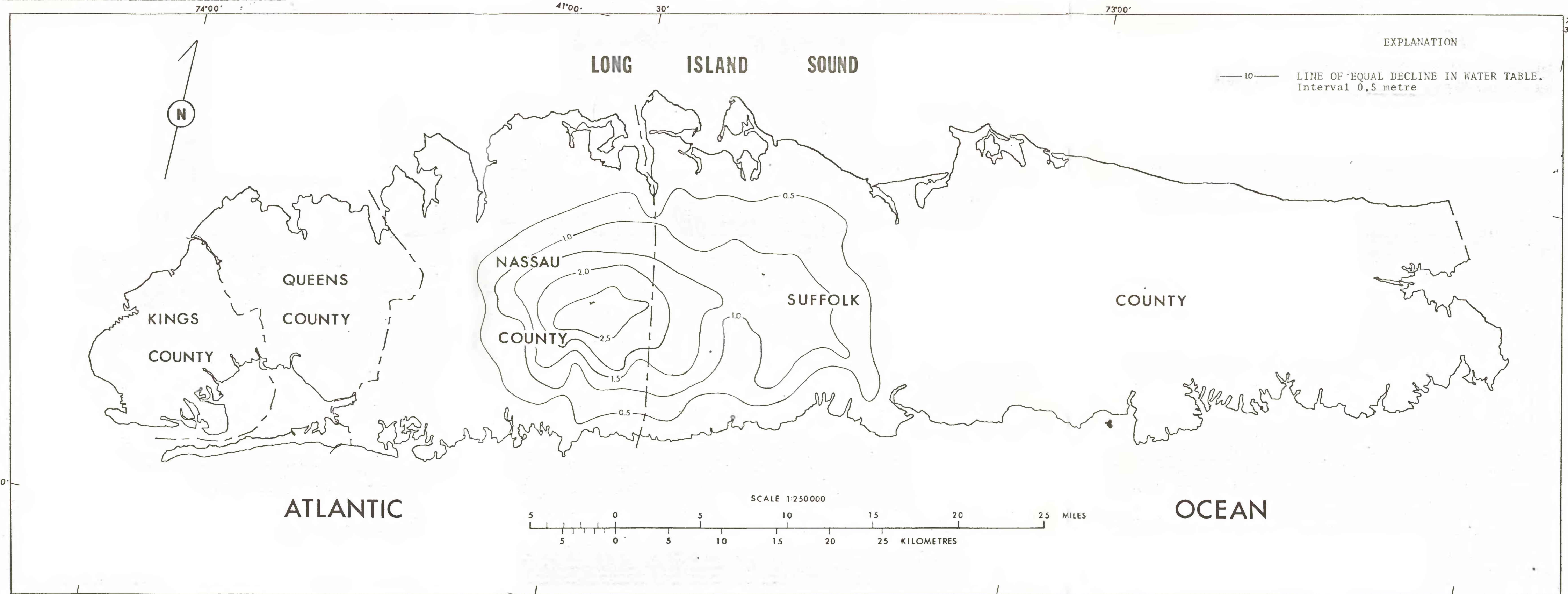
Figure 7.--Estimated water-table decline resulting from proposed sewer construction in Nassau and Suffolk Counties, Long Island, New York from 1975 to 1987.
