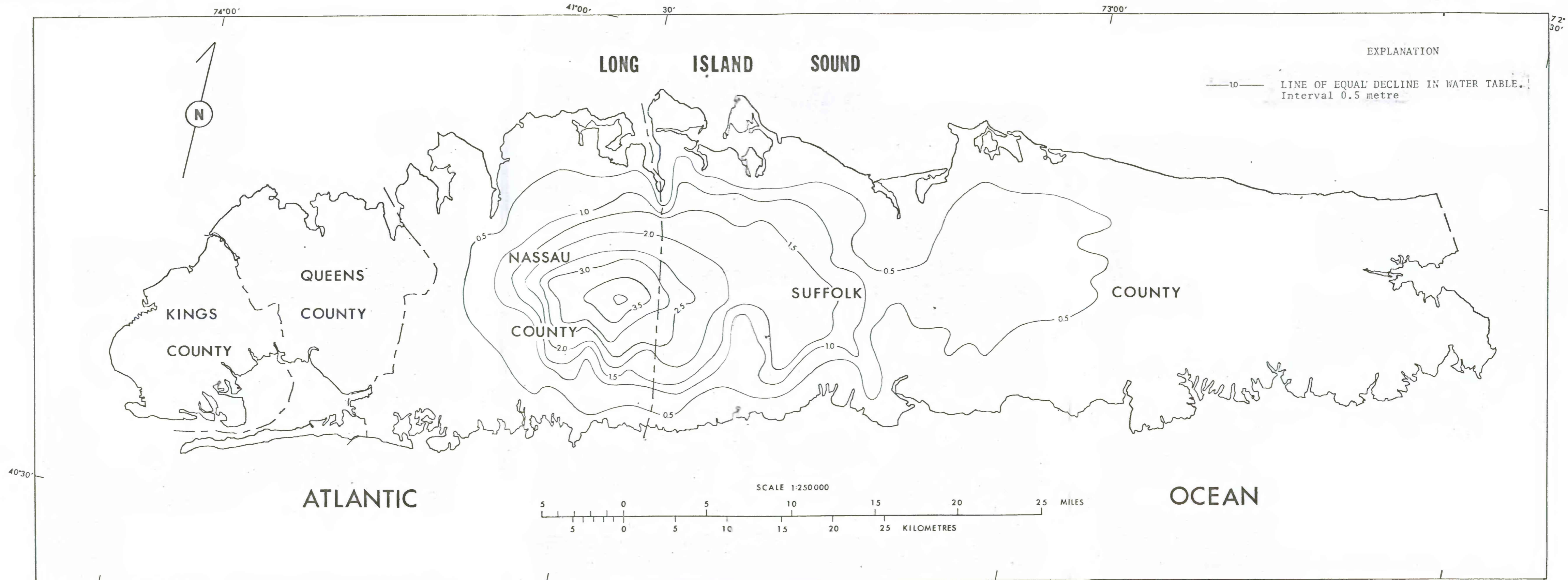
Figure 8.--Estimated water-table decline resulting from proposed sewer construction in Nassau and Suffolk Counties, Long Island, New York from 1975 to 1990.
