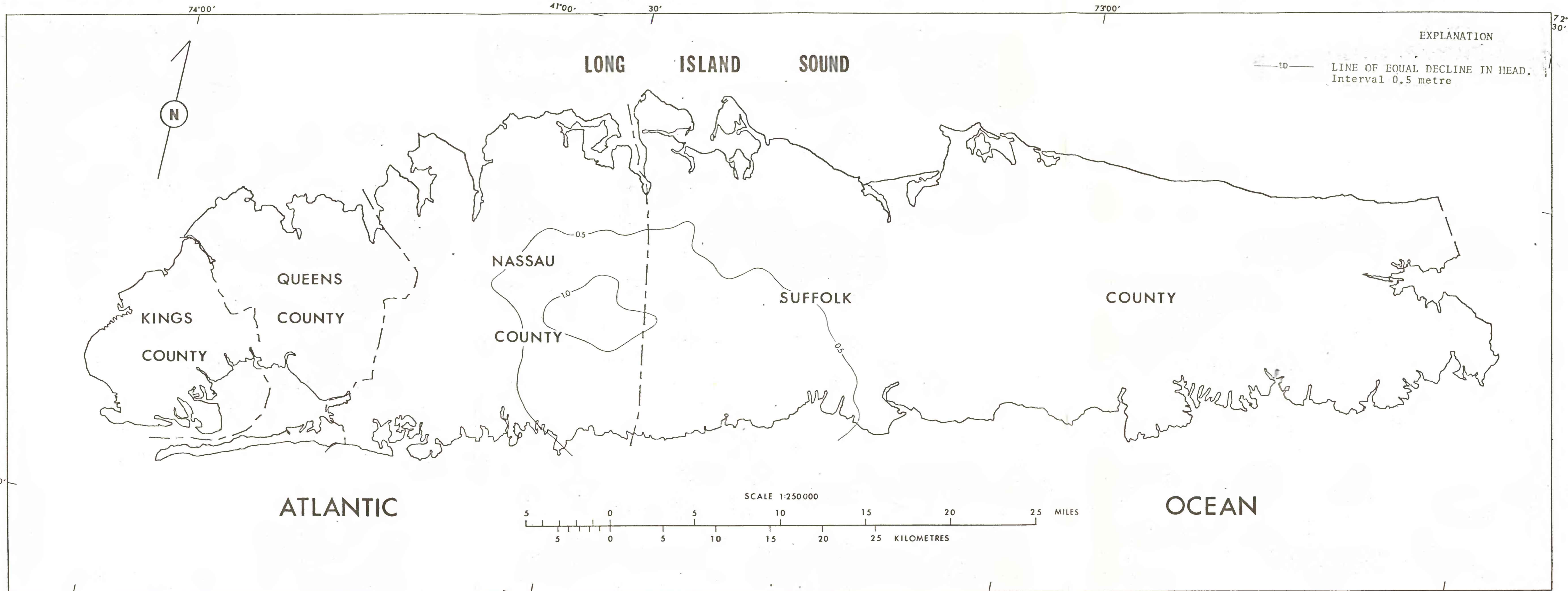
Figure 9.--Estimated head decline in Magothy aquifer resulting from proposed sewer construction in Nassau and Suffolk Counties, Long Island, New York from 1975 to 1984.
