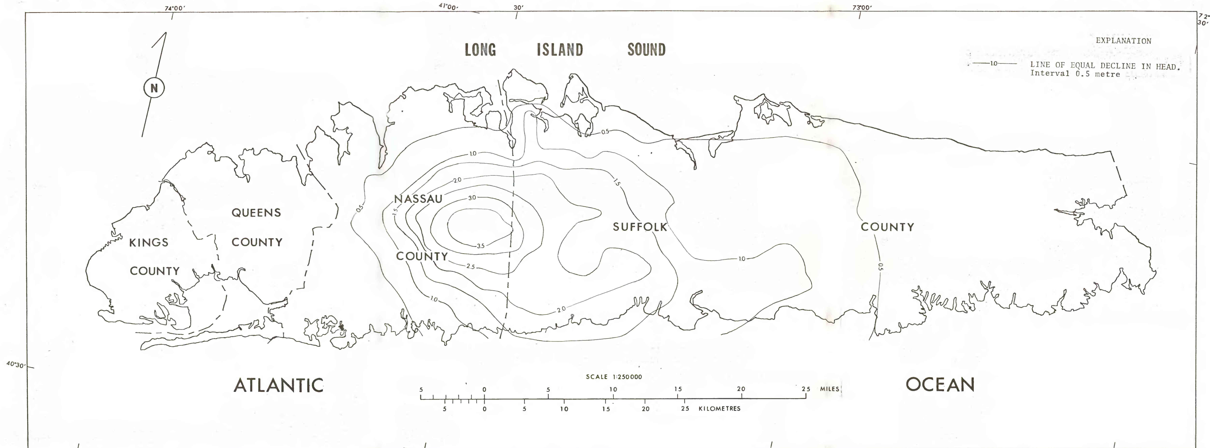
Figure 11.--Estimated head decline in Magothy aquifer resulting from proposed sewer construction in Nassau and Suffolk Counties, Long Island, New York from 1975 to 1990.
