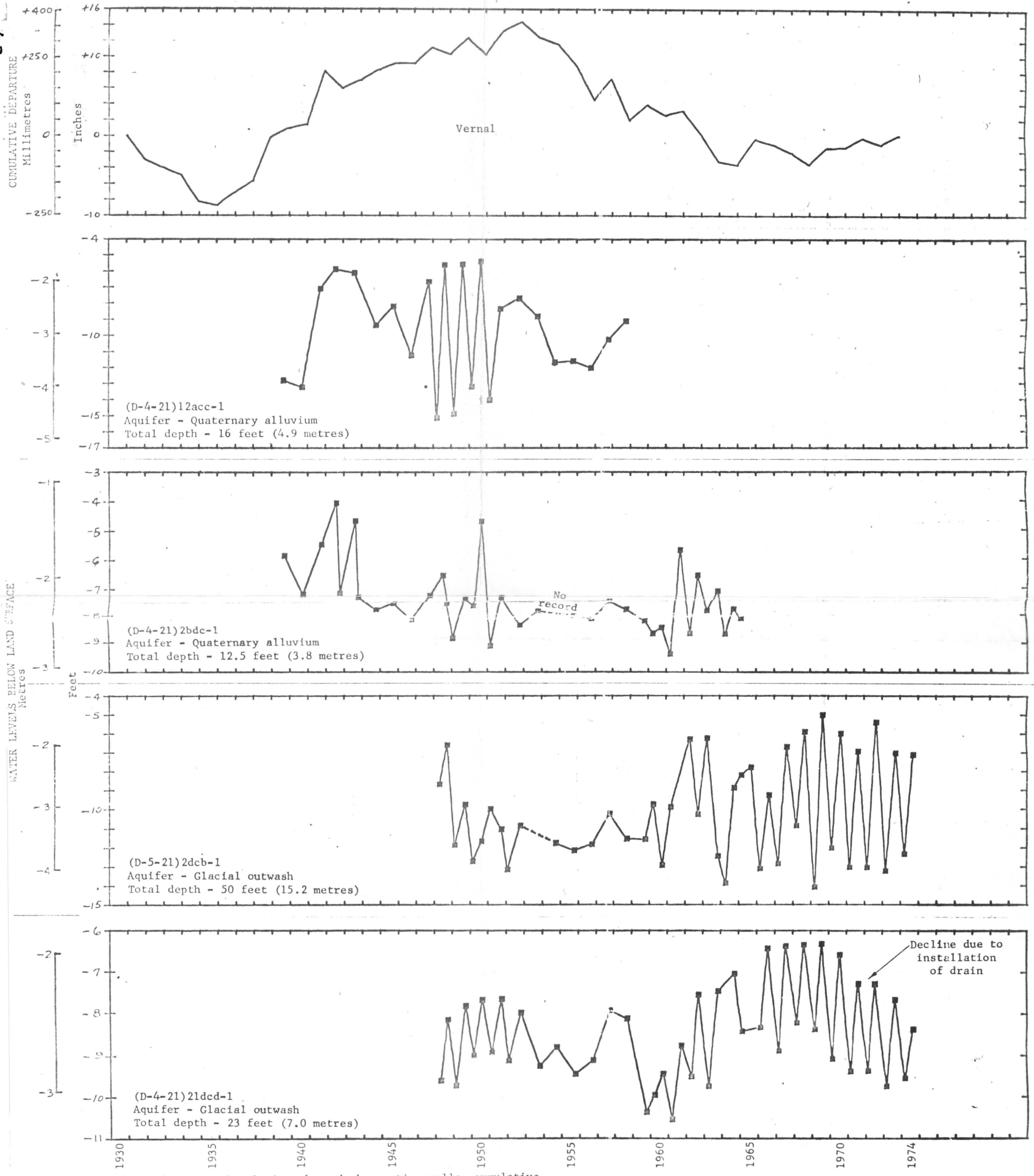
Figure 6.--Water levels in selected observation wells, cumulative departure from the 1931-73 average annual precipitation at Vernal and Jensen, and monthly discharge of Ashley Creek at station 09271500.
