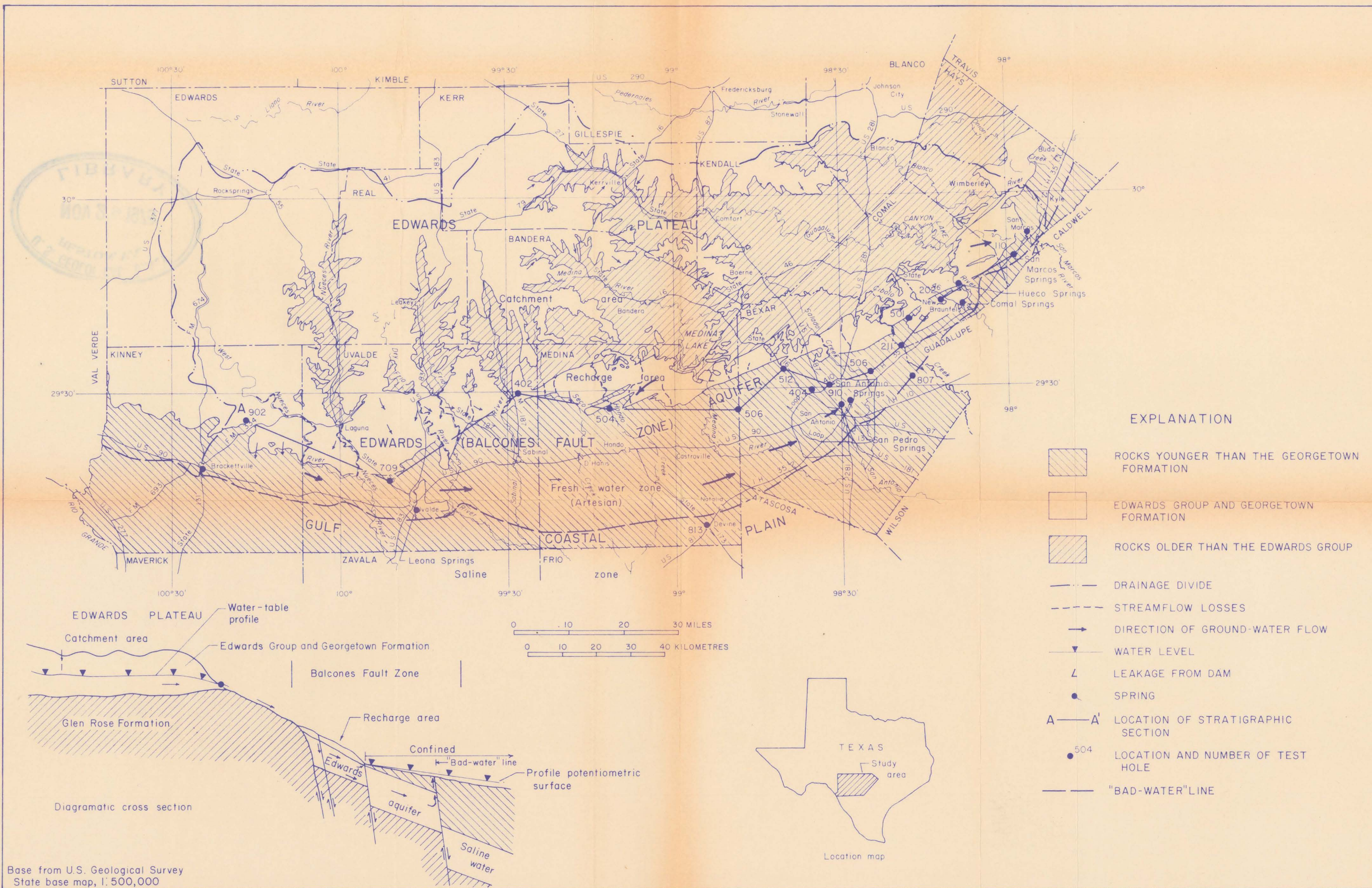
FIGURE 1.-Regional extent of the Edwards aquifer
