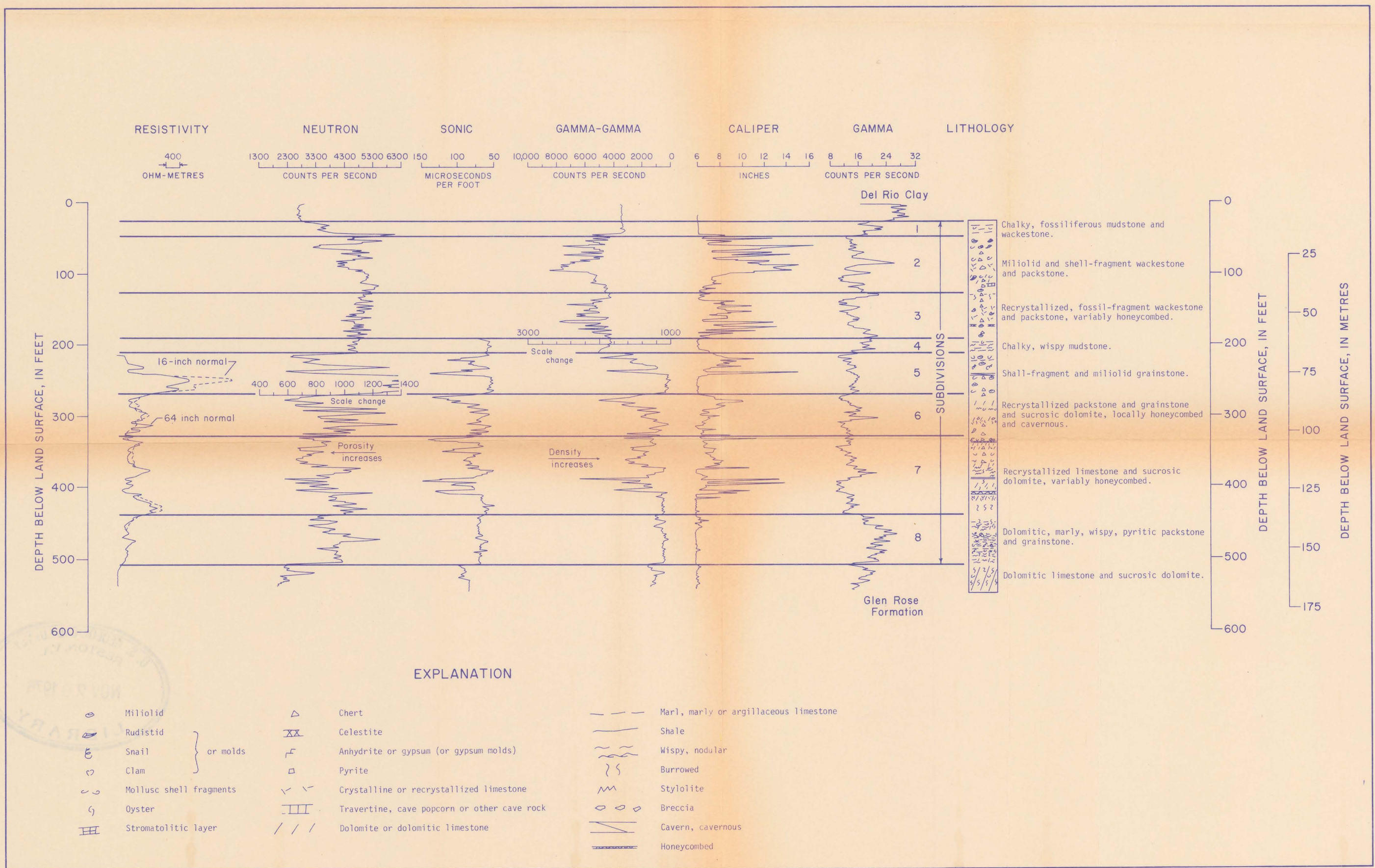
FIGURE 10.-Geophysical logs of the Lockhill test hole, AY 68-28-404
