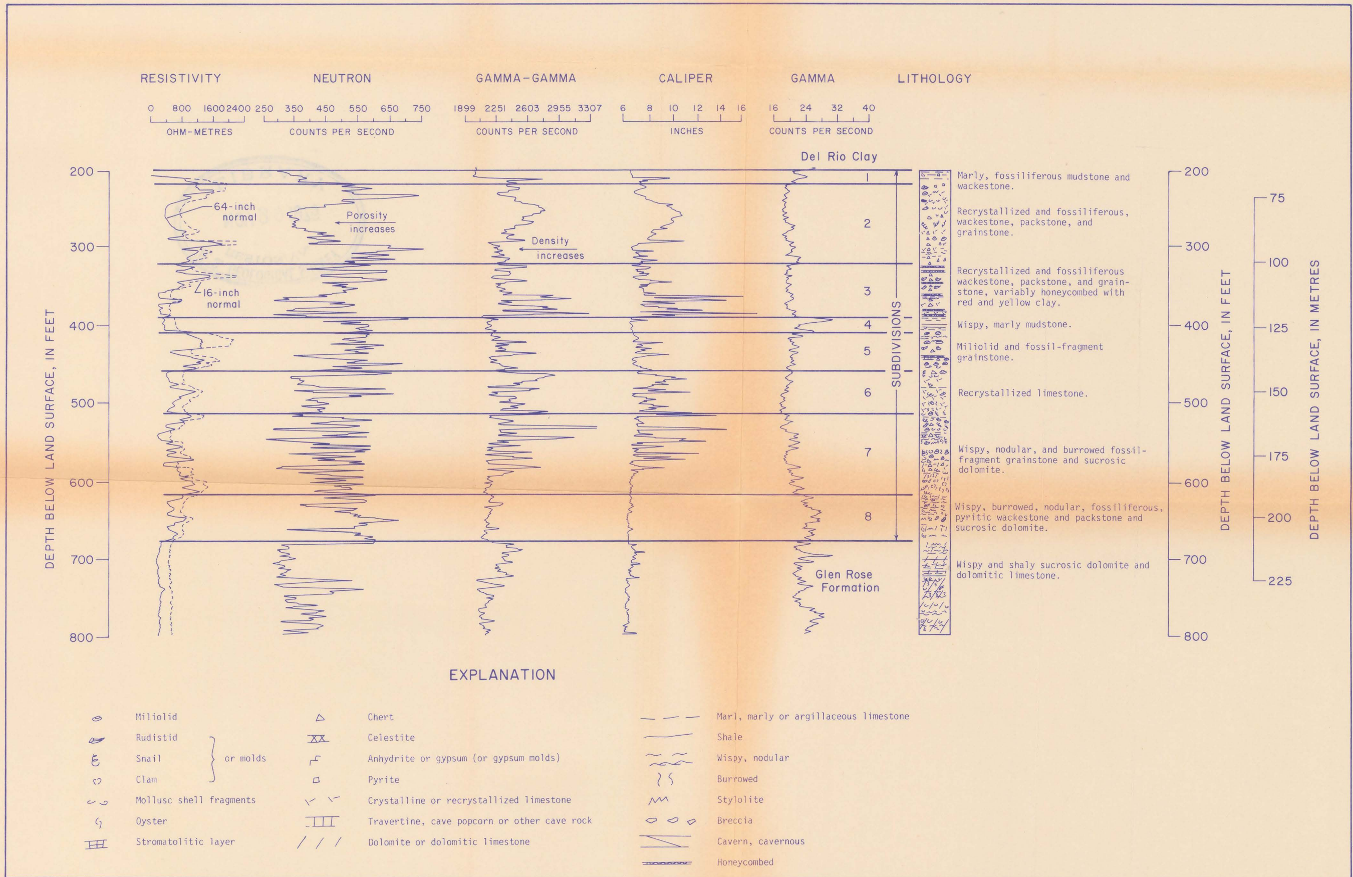
FIGURE 11.-Geophysical logs of the Castle Hills test hole, AY 68-28-910
