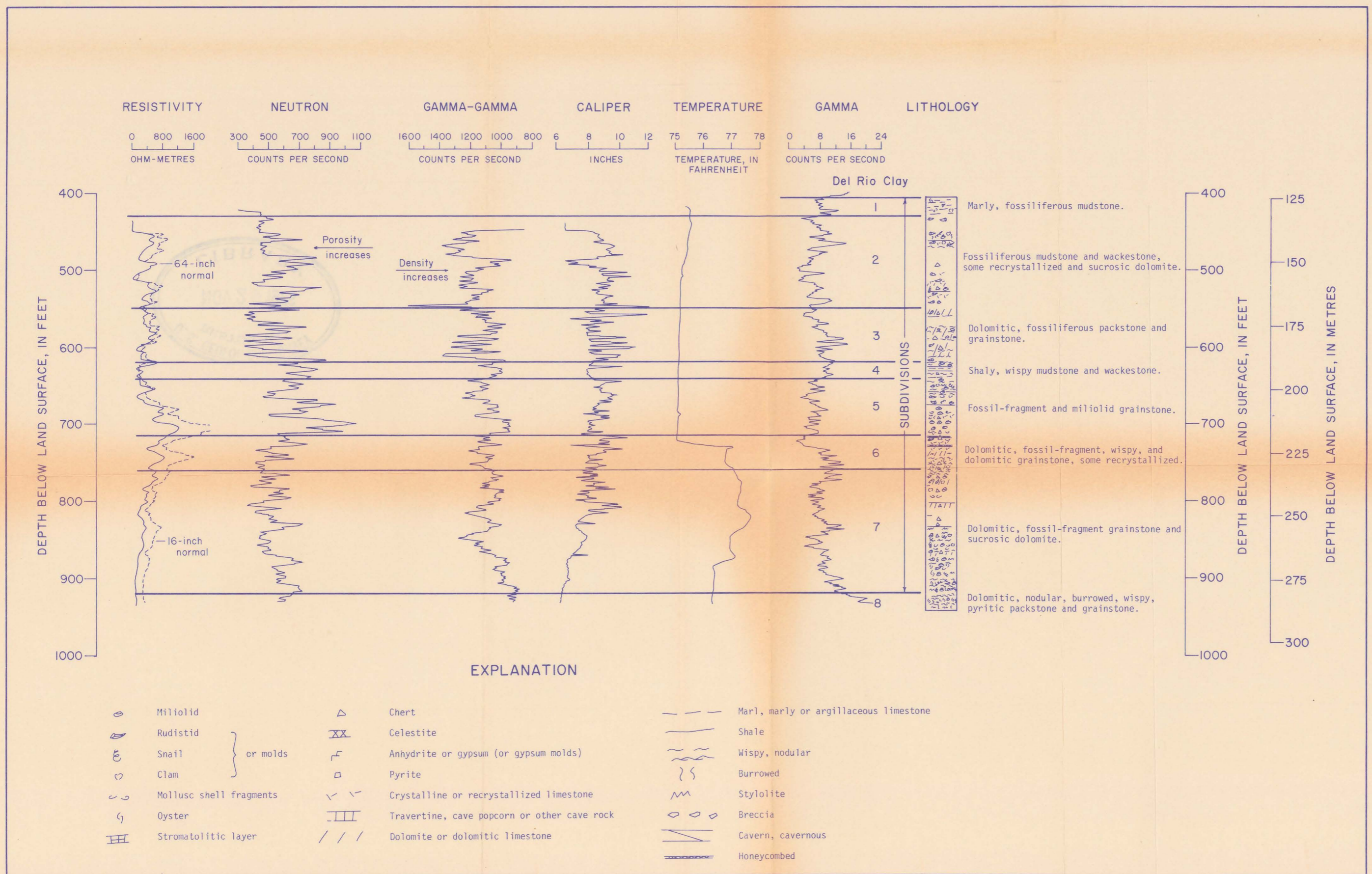
FIGURE 13.-Geophysical logs of the Rio Medina test hole, TD68-34-506
