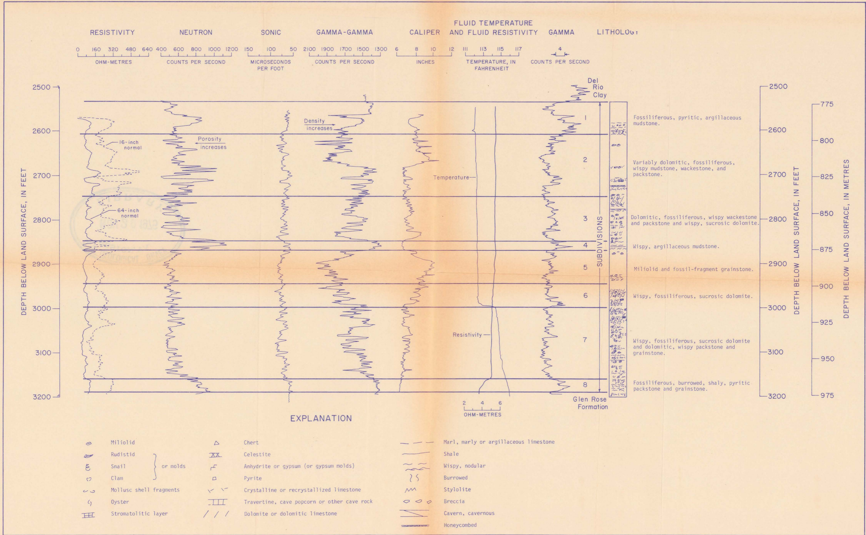
FIGURE 14.-Geophysical logs of the Devine test hole, TD 68-49-813
