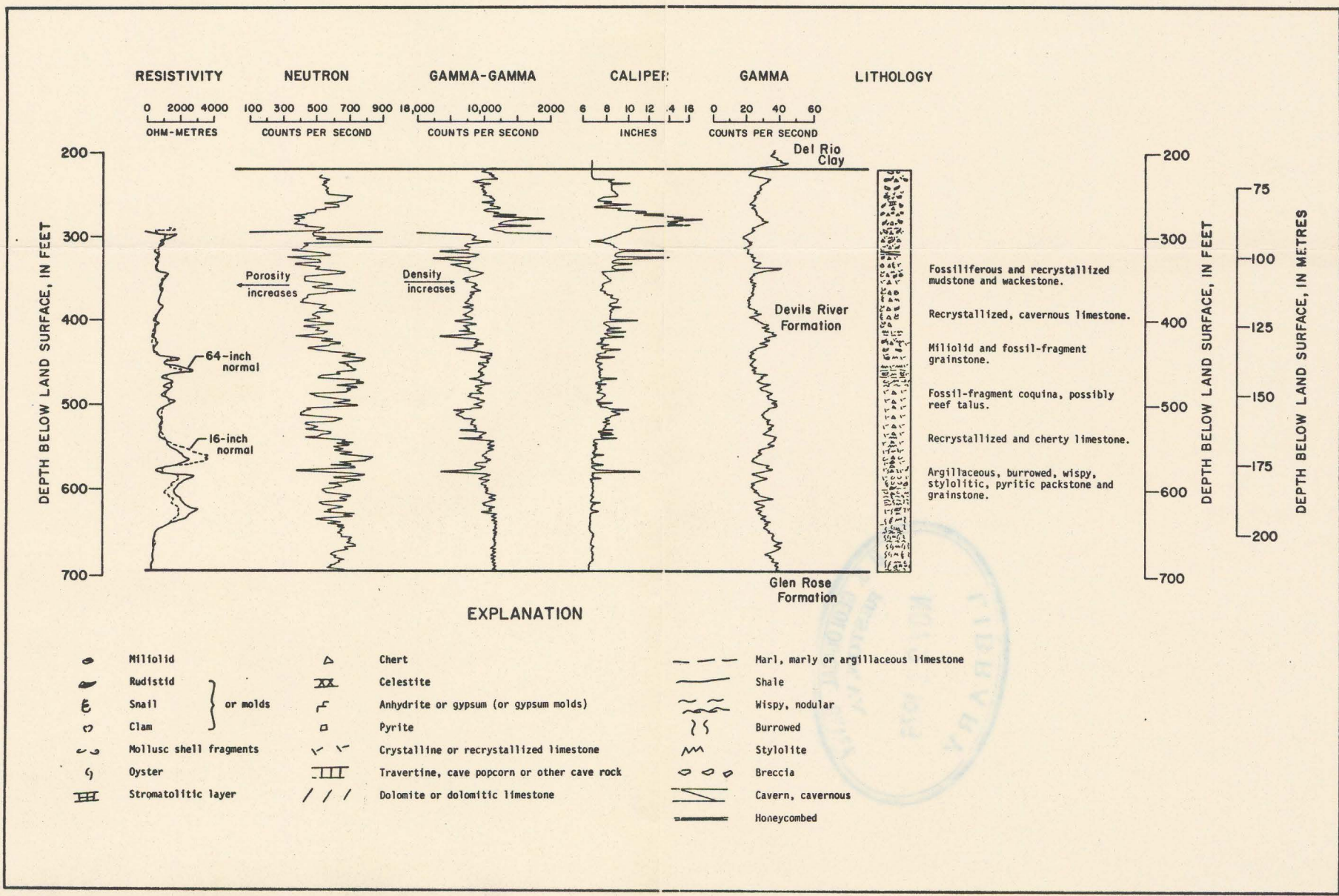
FIGURE 15.-Geophysical logs of the Sabinal test hole, YP 69-37-402
