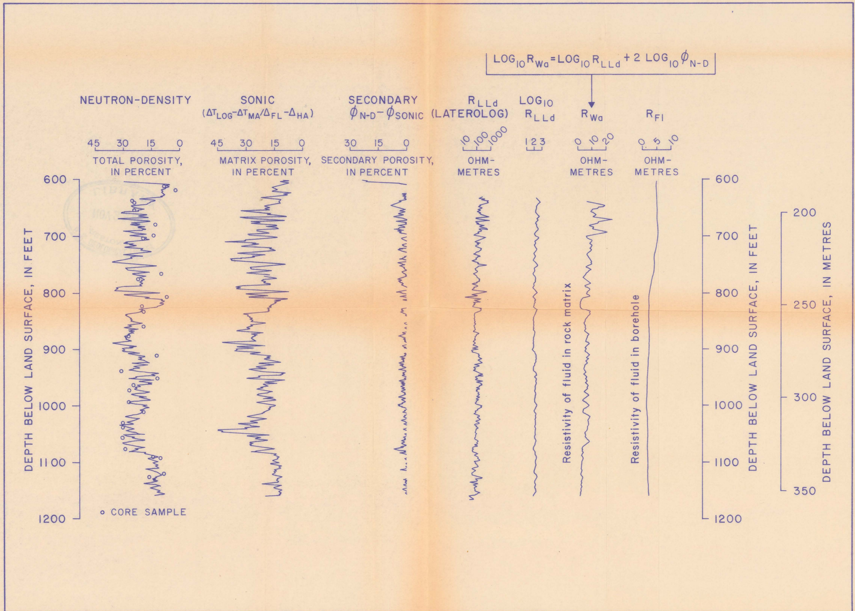
FIGURE 16.-Calculated secondary porosity and fluid resistivity at the Randolph test hole
