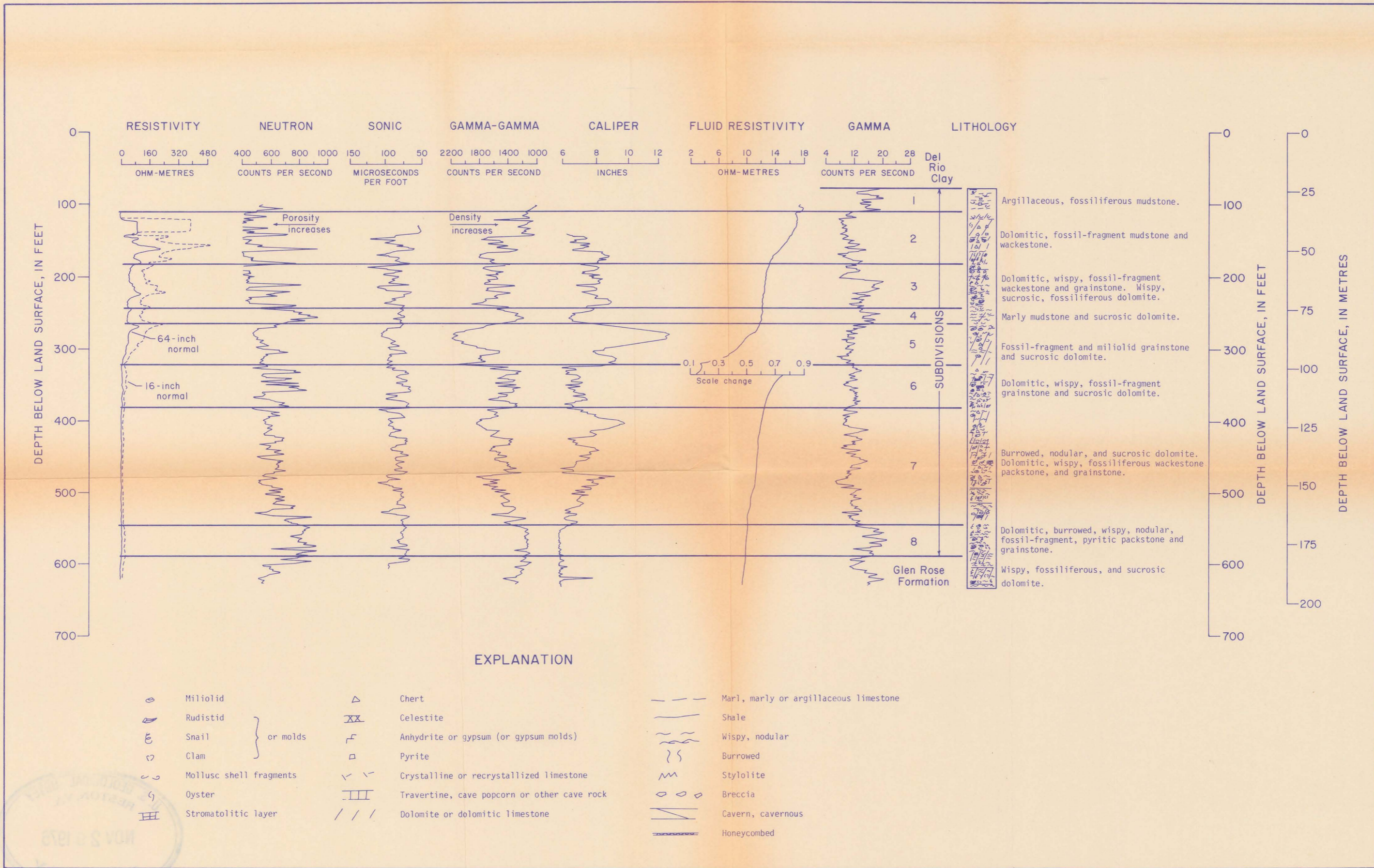
FIGURE 7.-Geophysical logs of the San Marcos test hole, LR 67-09-110
