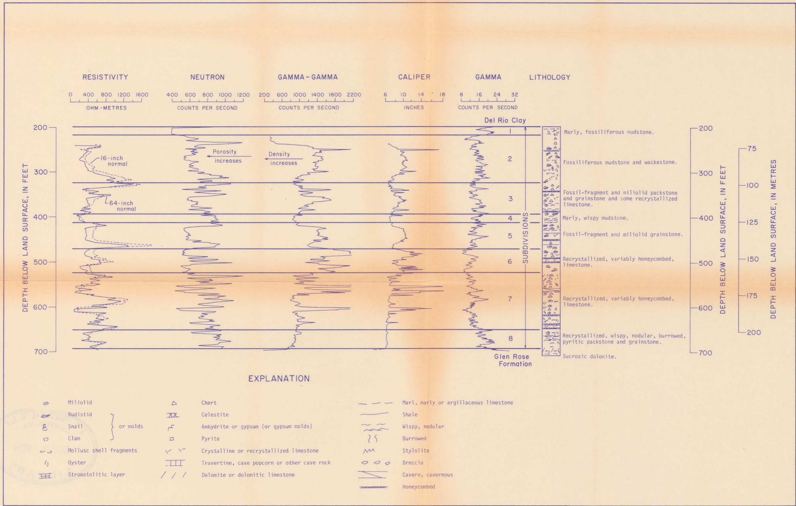
FIGURE 9.-Geophysical logs of the Feathercrest test hole, AY 68-29 -506
